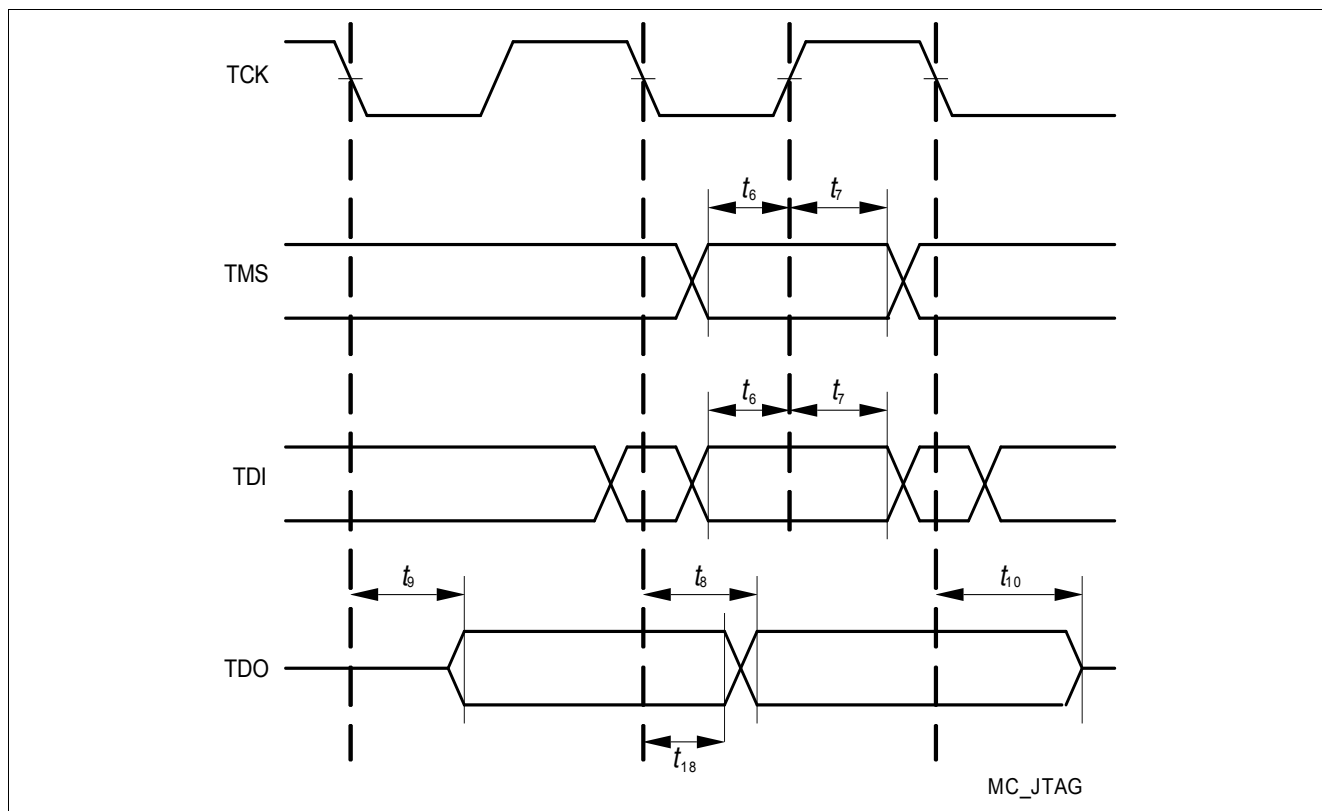
Figure 3-8 JTAG Timing
