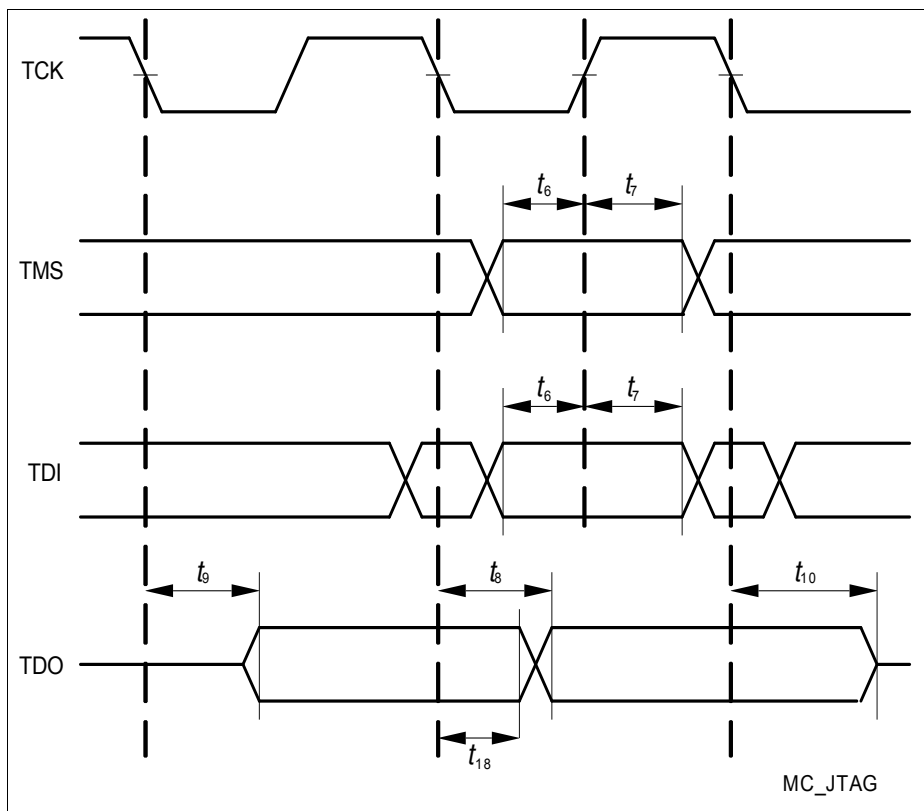
Figure 17 JTAG Timing
