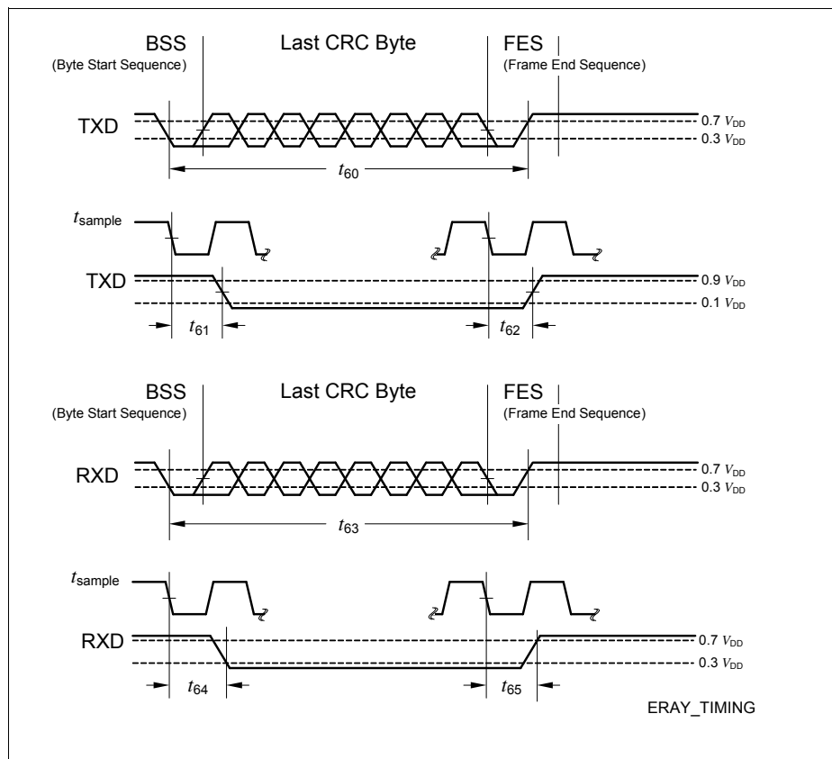
Figure 25 ERAY Timing
