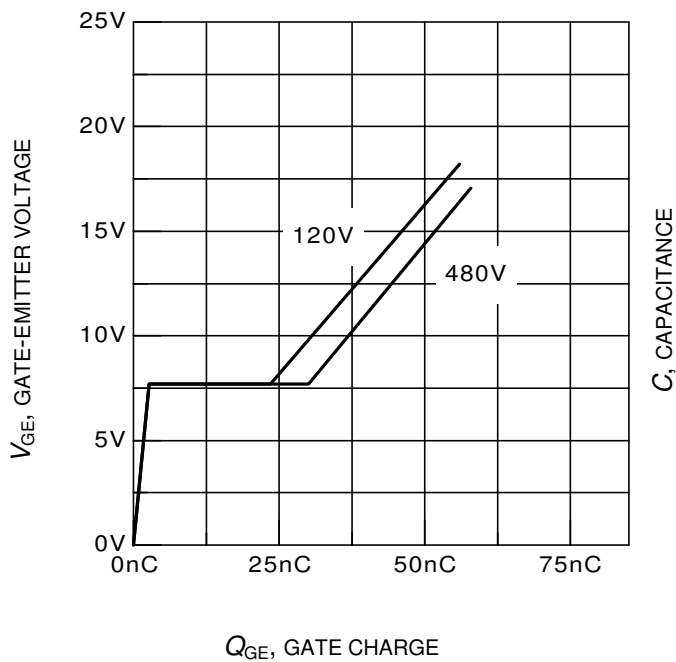
Figure 17. Typical gate charge ( I_C = 10A )
