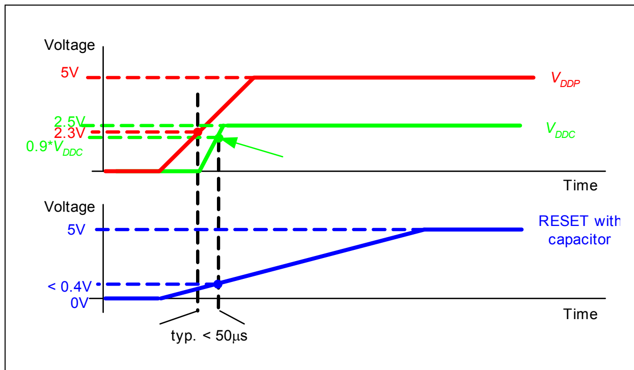
Figure 23 V_{DDP} , V_{DDC} and V_{RESET} during Power-on Reset
