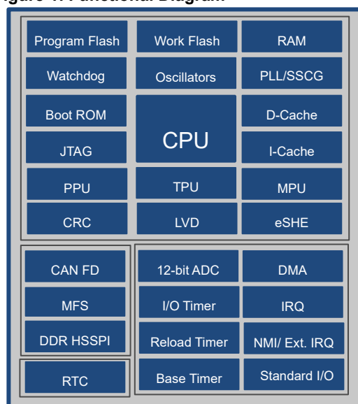
Figure 1: Functional Diagram
