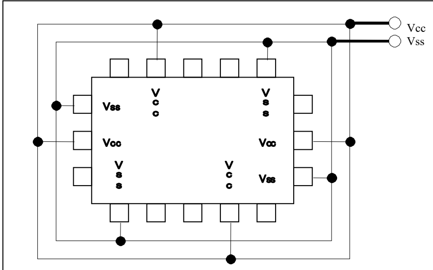
Figure 1-1 Pin Assignment
