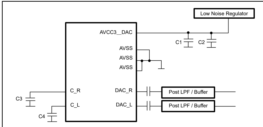
Figure 9-3: Coupling Capacitance (Example)
