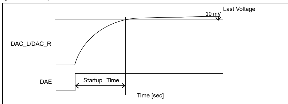
Figure 8-7: Startup Time
