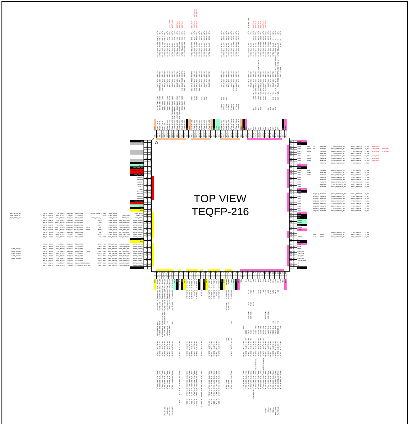
Figure 4-8: TEQFP-216 (S6J32KELxx)
