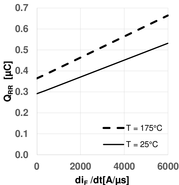
Figure 19 Typical reverse recovery charge as a function of diode current slope (Q_{rr} = f(di_t/dt), V_{DD} = 800V, V_{GS} = 0V/18V, I_D = 25A, \text{ind. load, test circuit in Fig. E, body diode at } V_{GS} = 0V)
