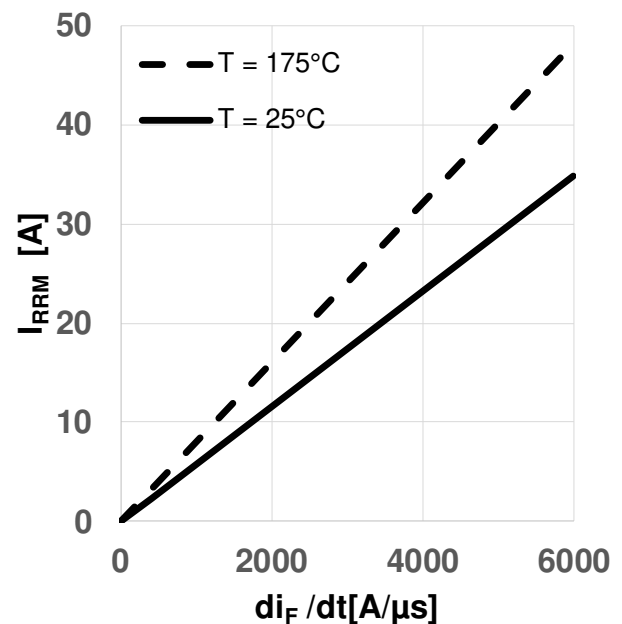
Figure 20 Typical reverse recovery current as a function of diode current slope (I_{rrm} = f(di_t/dt), V_{DD} = 800V, V_{GS} = 0V/18V, I_D = 25A, \text{ind. load, test circuit in Fig. E, body diode at } V_{GS} = 0V)
