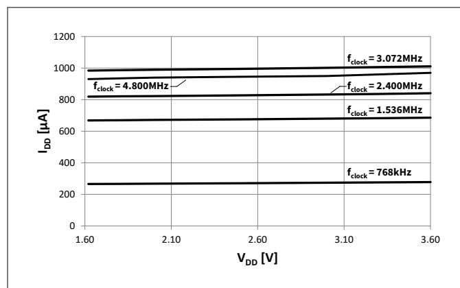
Figure 8 Typical I_{\text{DD}} vs V_{\text{DD}}
