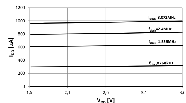
Plot 5: I_{DD} vs. V_{DD}
