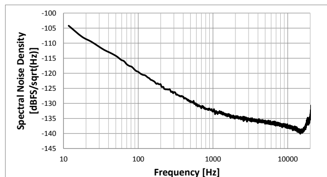
Plot 6: Typical noise floor (unweighted)
