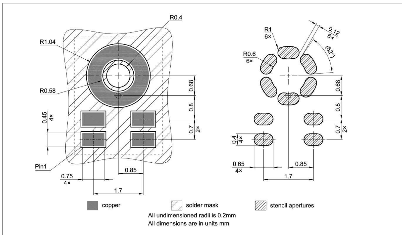
Figure 8 Footprint and stencil recommendation
