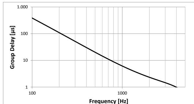
Plot 4: Typical group delay vs. frequency
