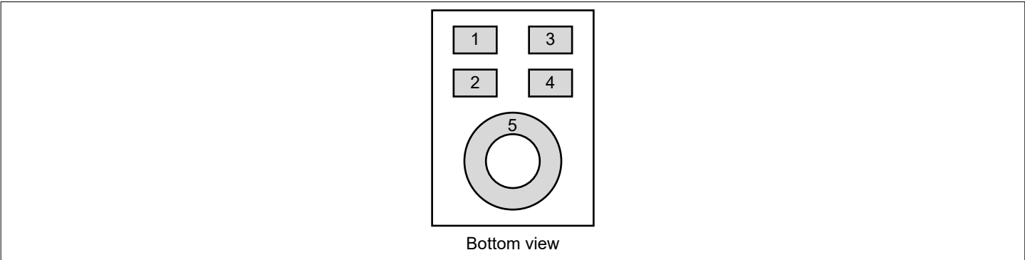
Figure 2 Pin configuration
