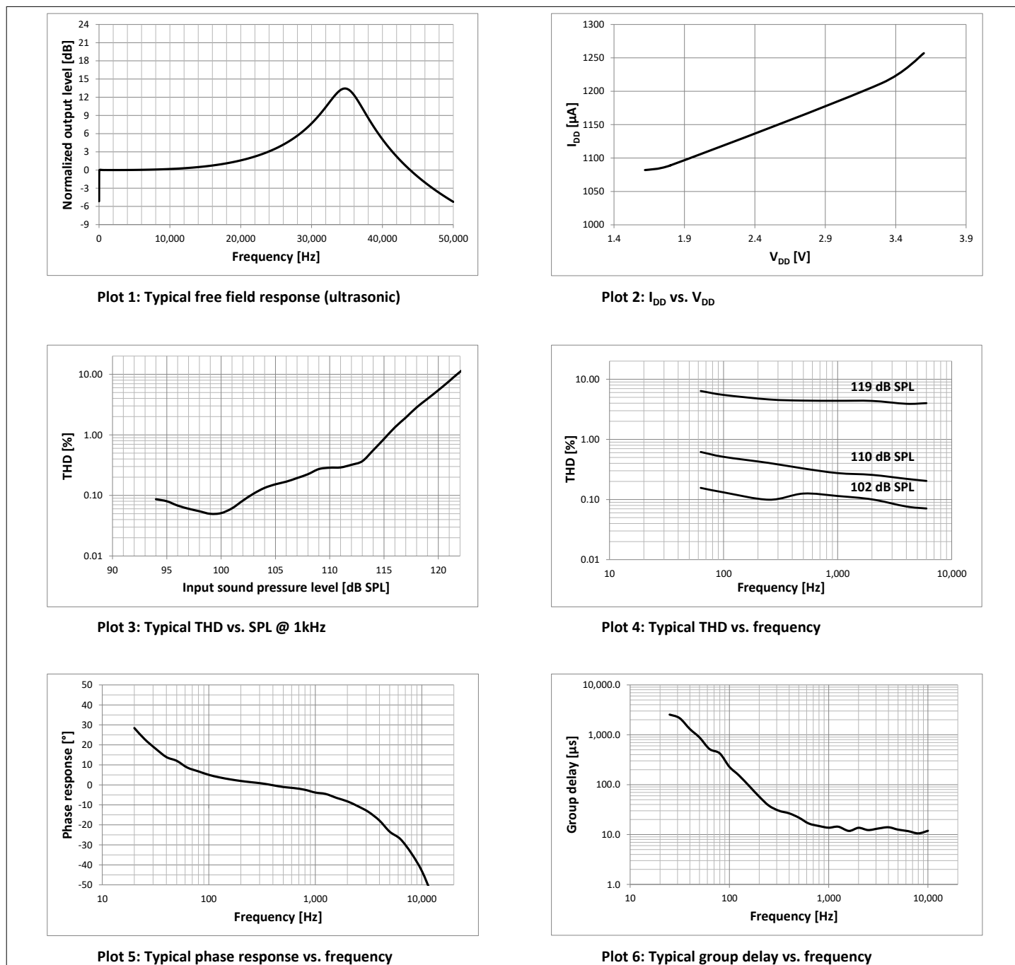
Figure 5 Typical performance characteristics
