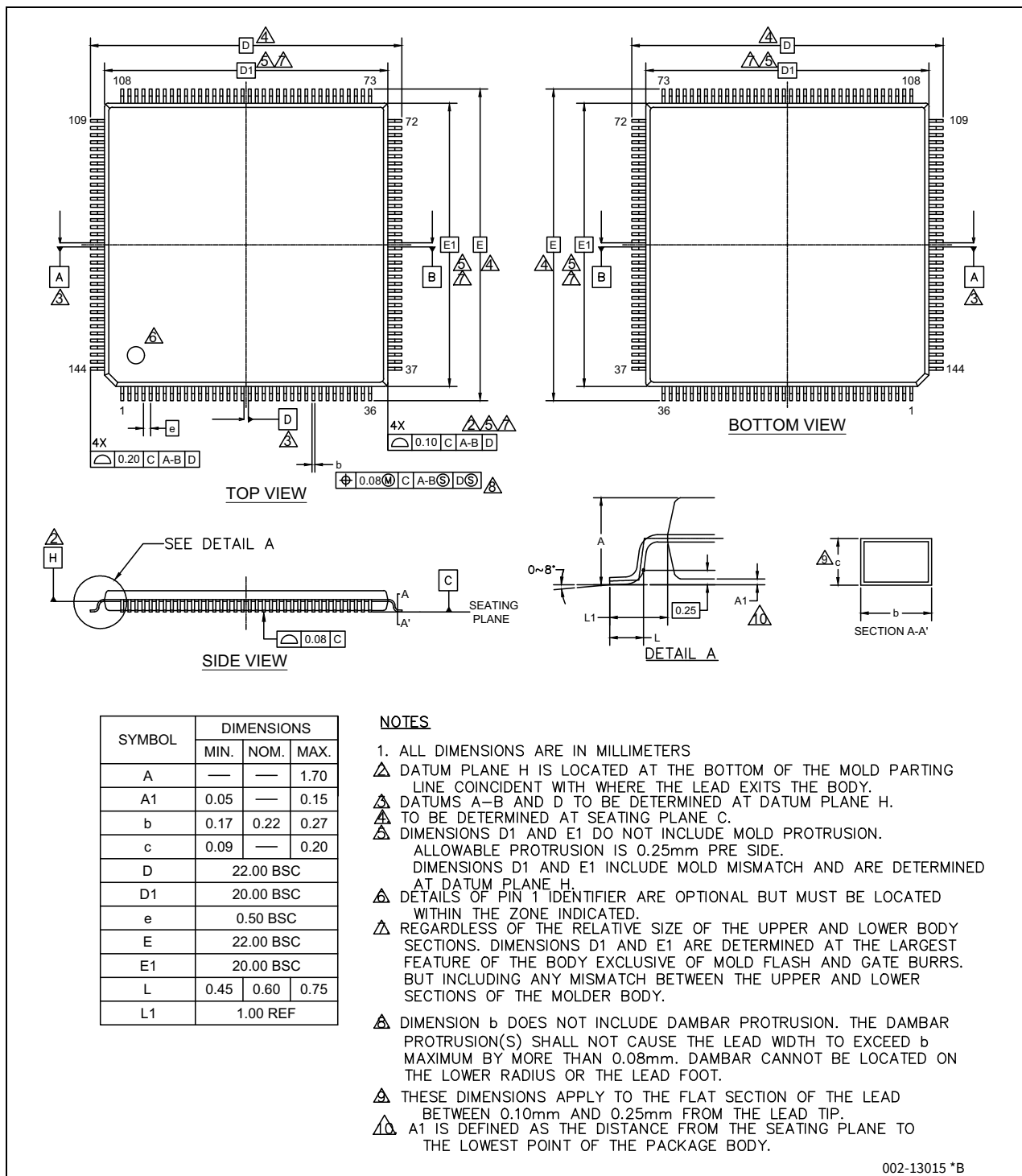
Figure 28-2 Package Outline - 144-LQFP
