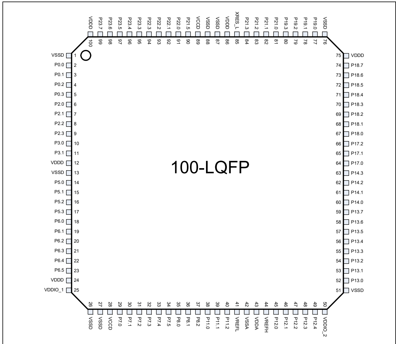
Figure 9-5 100-LQFP pin assignment
