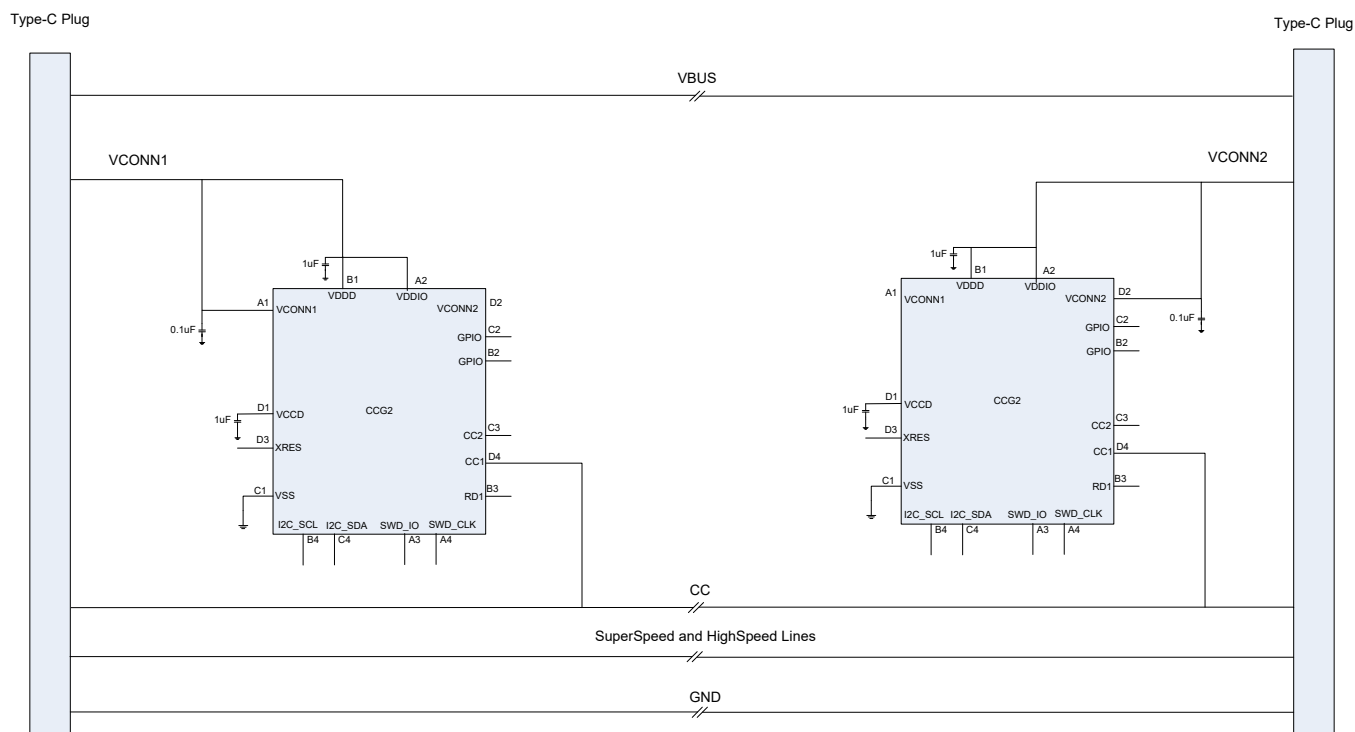
Figure 10. Passive EMCA Application – Single EZ-PD CCG2 Per Plug (VCONN range between 2.7V to 5.5V)
