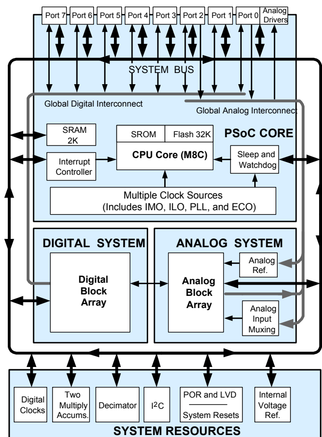
Figure 3-1. PSoC Architecture
