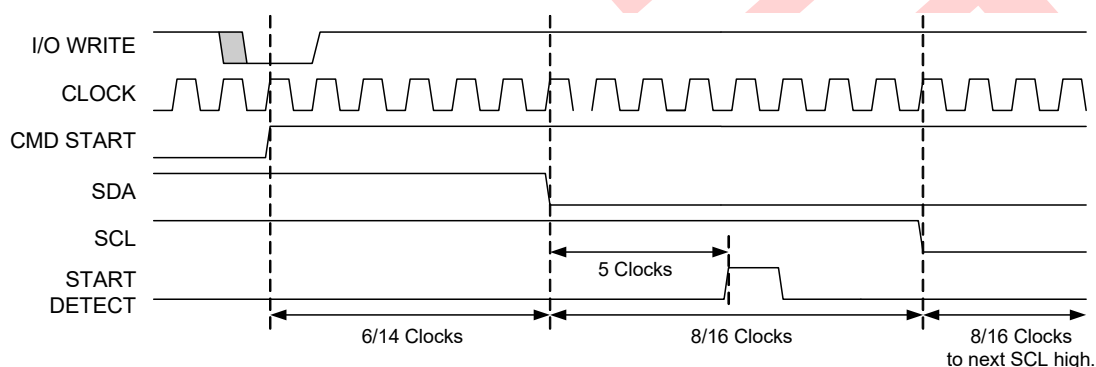
Figure 24-9. Basic Master Start Timing
