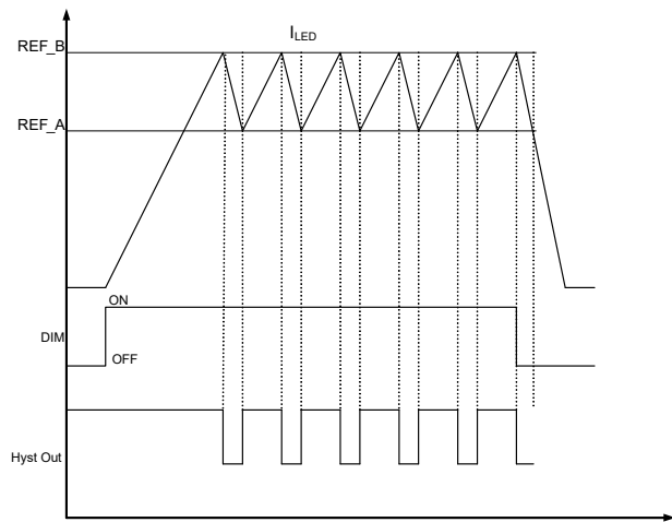
Current Waveforms
