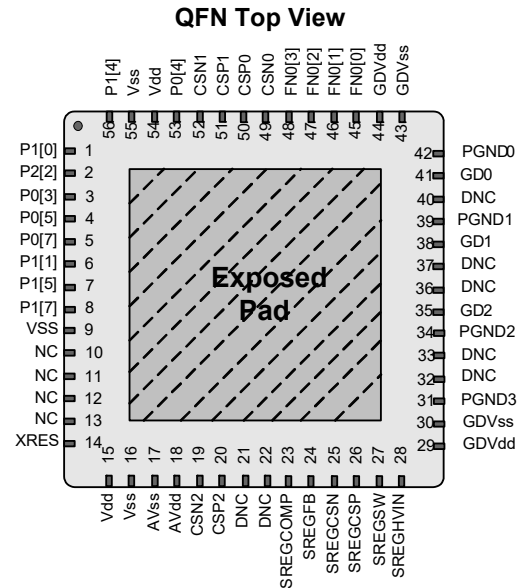
CY8CLED03G01 56-Pin PowerPSoC Device
