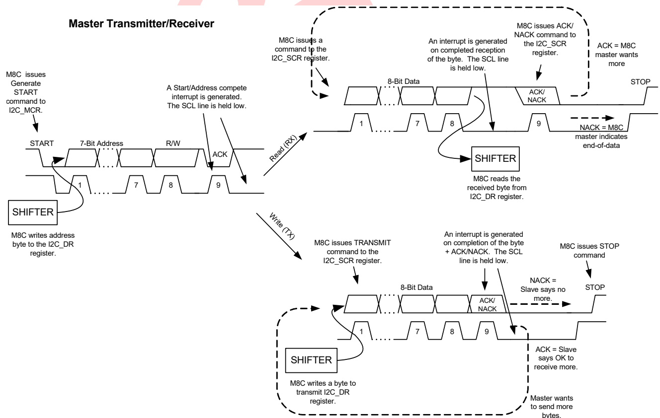
Figure 24-3. Master Operation
