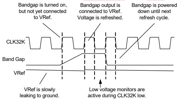
Figure 10-3. Bandgap Refresh Operation
