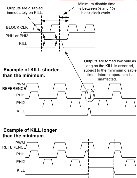
Figure 14-14. Asynchronous Restart Kill Mode
