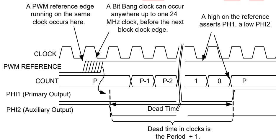
Figure 14-9. Basic Dead Band Timing
