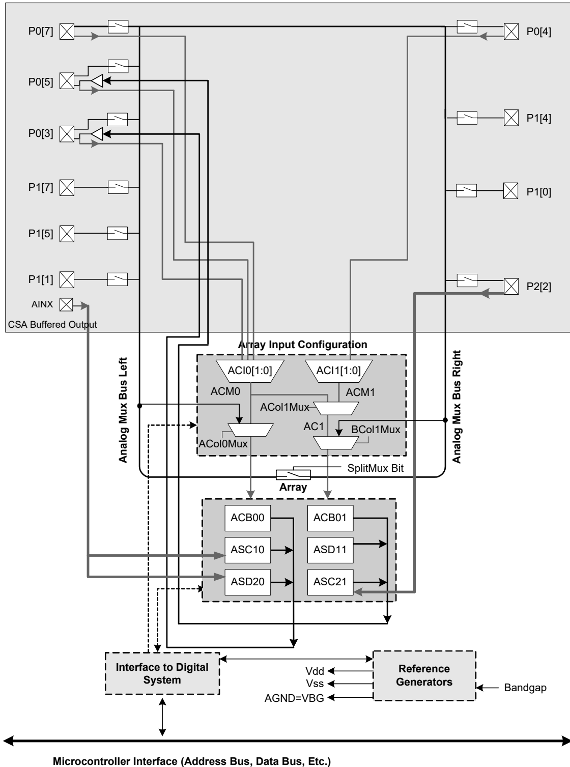
Figure 17-2. Two Column PSoC Analog Pin Block Diagram
