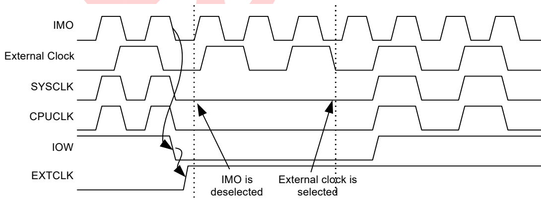
Figure 21-4. Switch from IMO to External Clock with the CPU Running with a CPU Clock Divider of One
