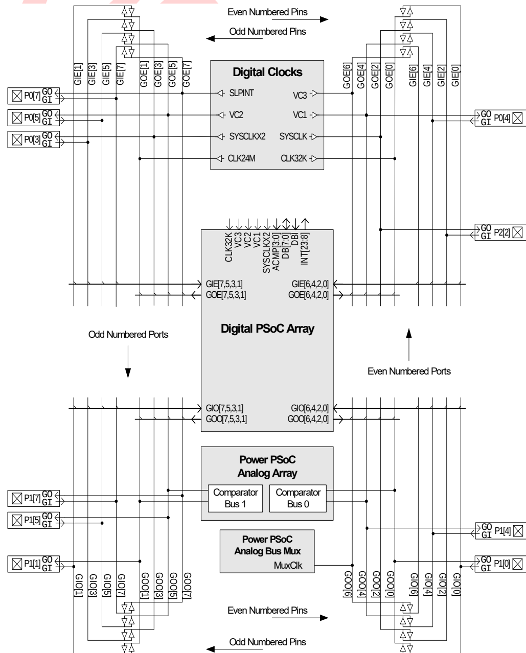
Figure 11-1. Global Interconnect Block Diagram for the 56-Pin Package
