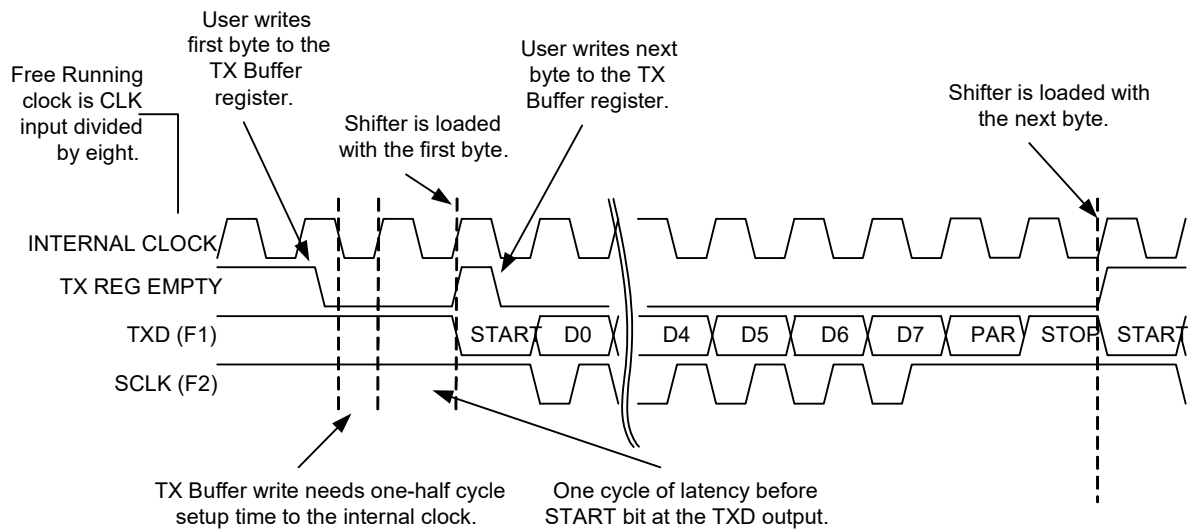
Figure 14-24. Typical Transmitter Timing
