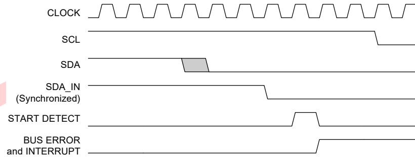
Figure 24-8. Bus Error Interrupt Timing
