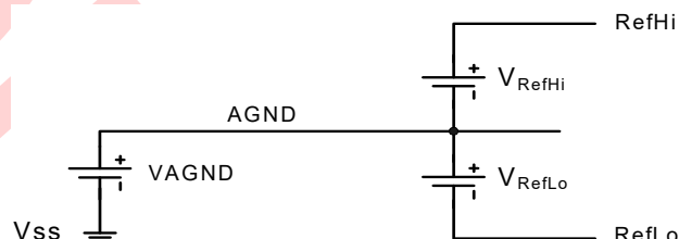
Figure 18-1. Analog Reference Structure
