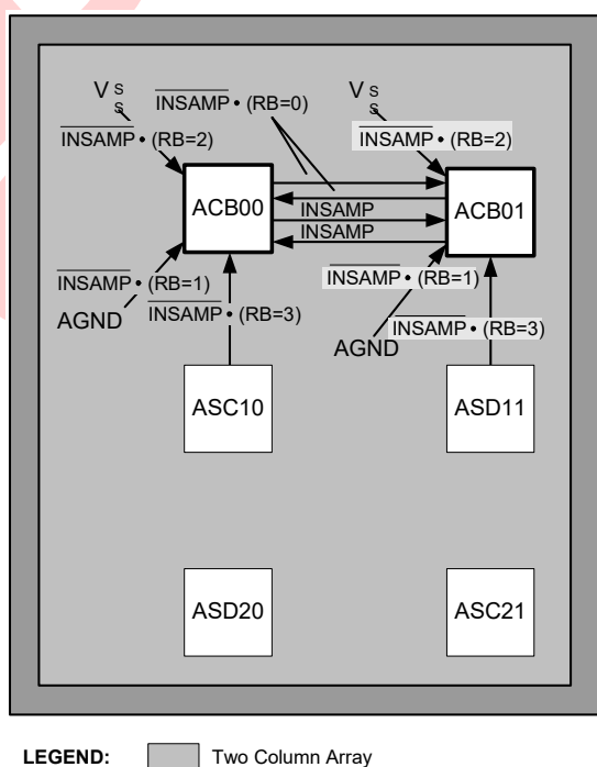
Figure 16-4. RBotMux Connections
