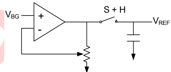
Figure 25-1. Voltage Reference Schematic
