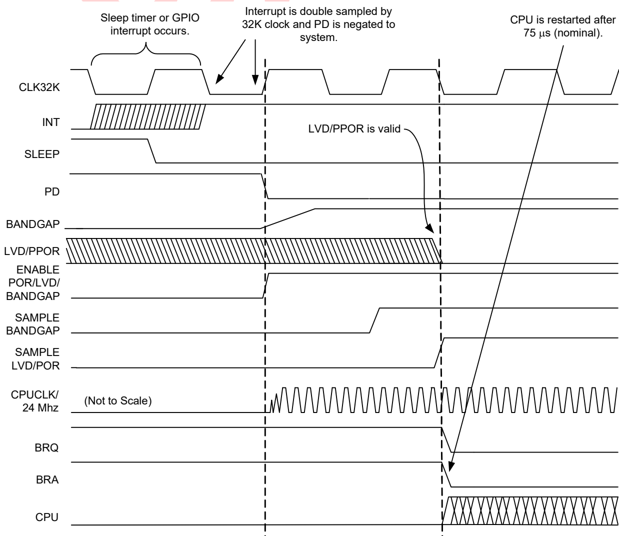
Figure 10-2. Wakeup Sequence
