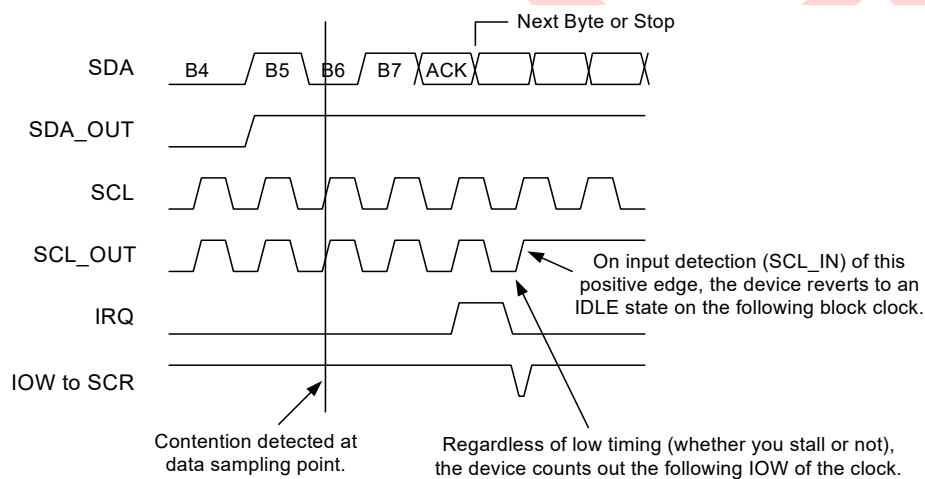
Figure 24-15. Lost Arbitration Timing (Transmitting Address or Data)
