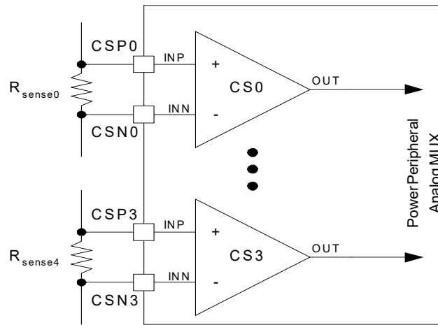
Figure 29-3. Four Independent Channels Example
