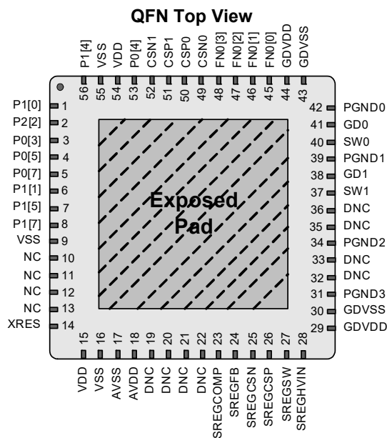
CY8CLED02D0x 56-Pin PowerPSoC Device
