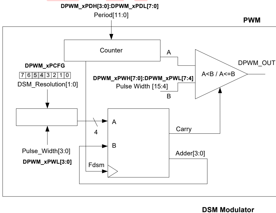
Figure 35-5. DMM Architecture
