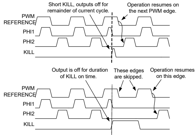
Figure 14-13. Synchronous Restart KILL Mode
