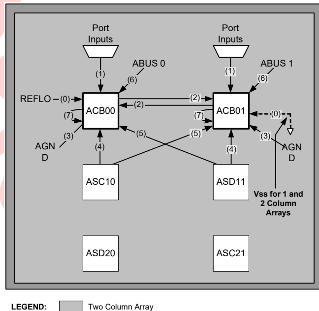
Figure 16-3. PMux Connections
