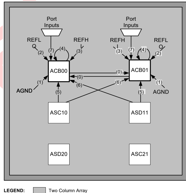
Figure 16-2. NMux Connections
