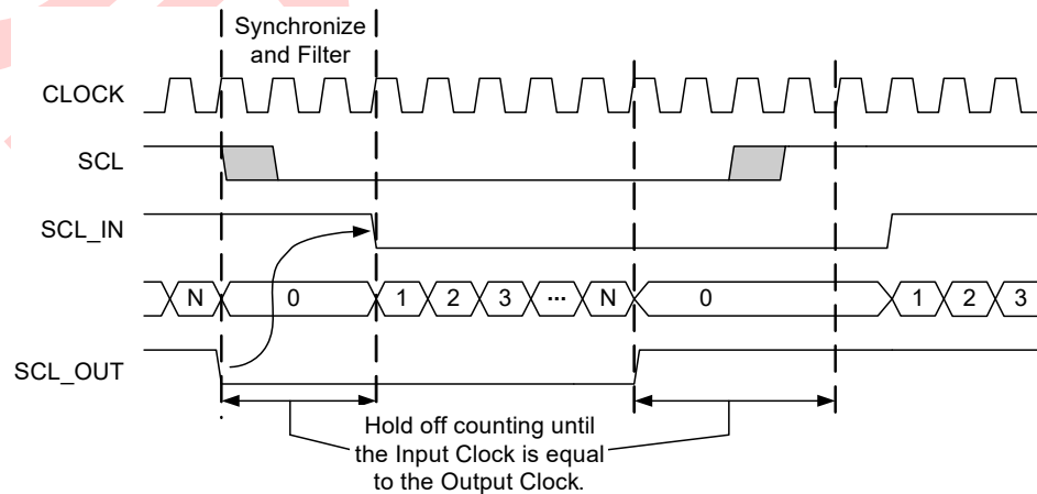
Figure 24-16. Master Clock Synchronization
