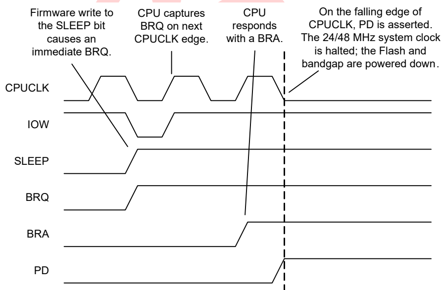
Figure 10-1. Sleep Sequence
