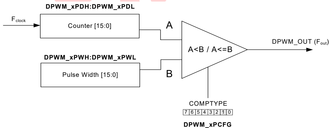
Figure 35-2. PWM Architecture
