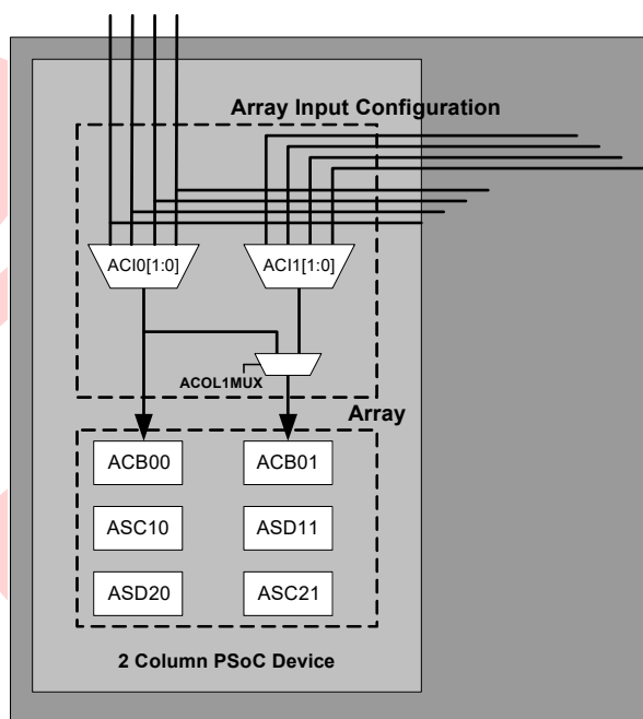
Figure 17-1. Analog Input Configuration Column Overview
