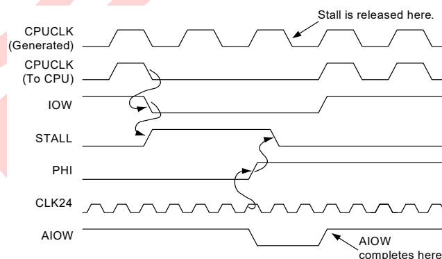
Figure 15-4. Synchronized Write to a DAC Register
