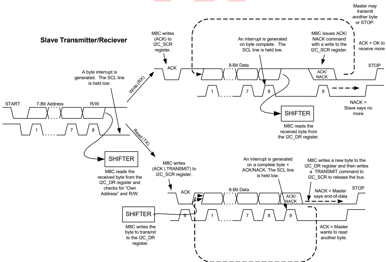
Figure 24-2. Slave Operation
