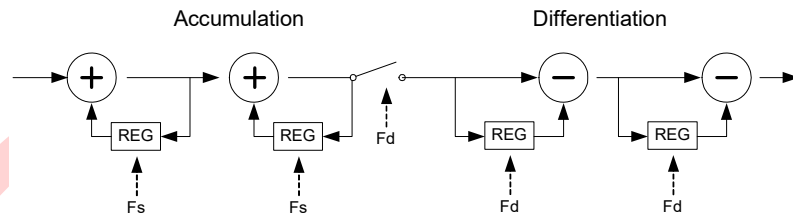
Figure 23-2. Sinc 2 Filter Block Diagram
