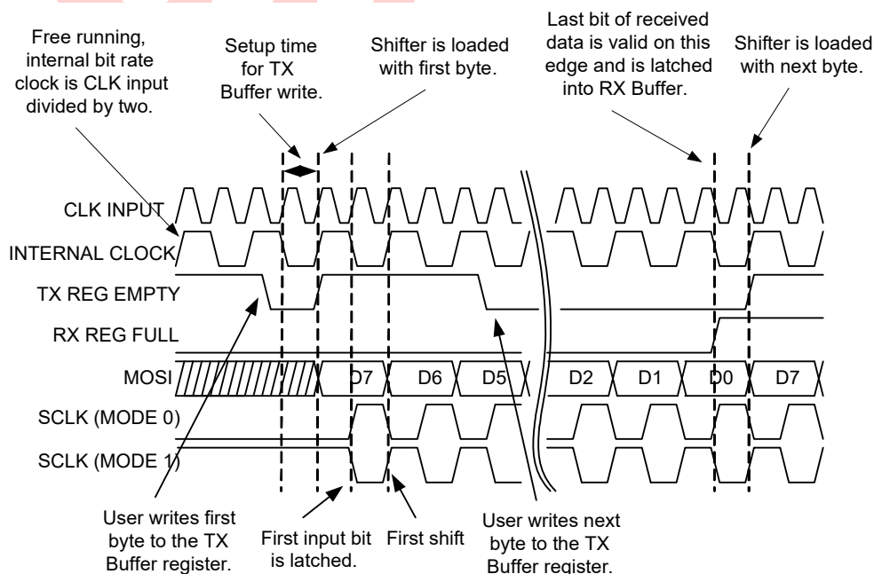
Figure 14-16. Typical SPIM Timing in Mode 0 and 1
