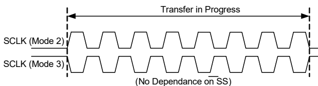
Figure 14-23. Mode 2 and 3 Transfer in Progress
