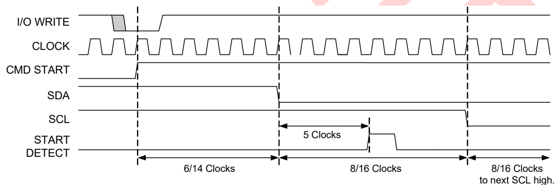
Figure 24-9. Basic Master Start Timing
