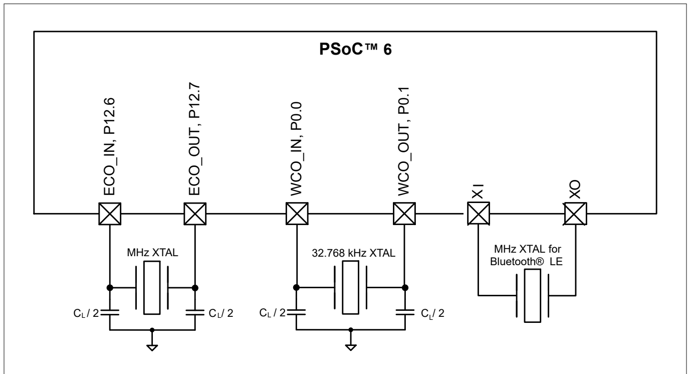
Figure 5 Oscillator circuits
