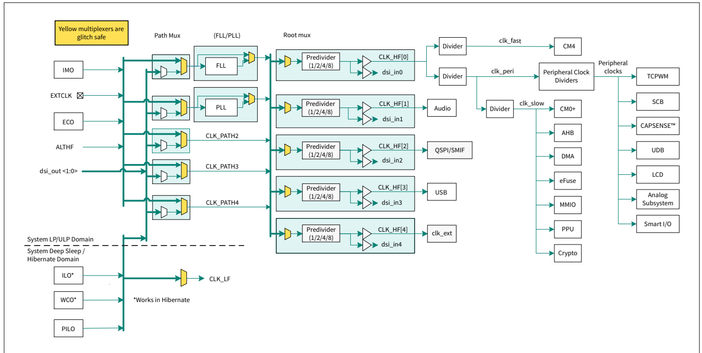
Figure 4 Clocking diagram
