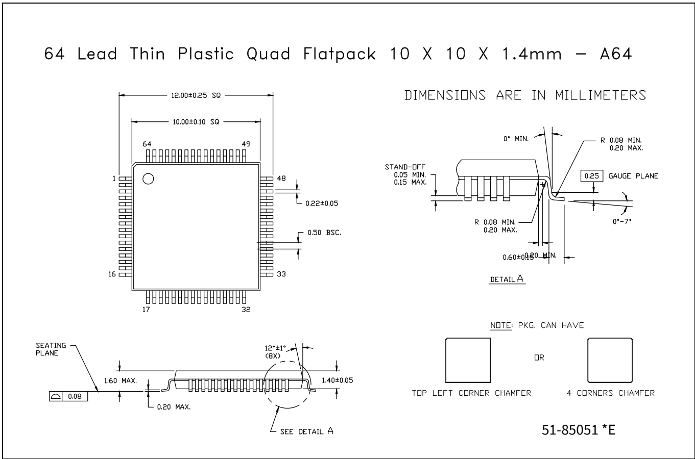
Figure 10 64-pin TQFP (10 × 10 × 1.4 mm) A64SB package outline (PG-TQFP-64), 51-85051
