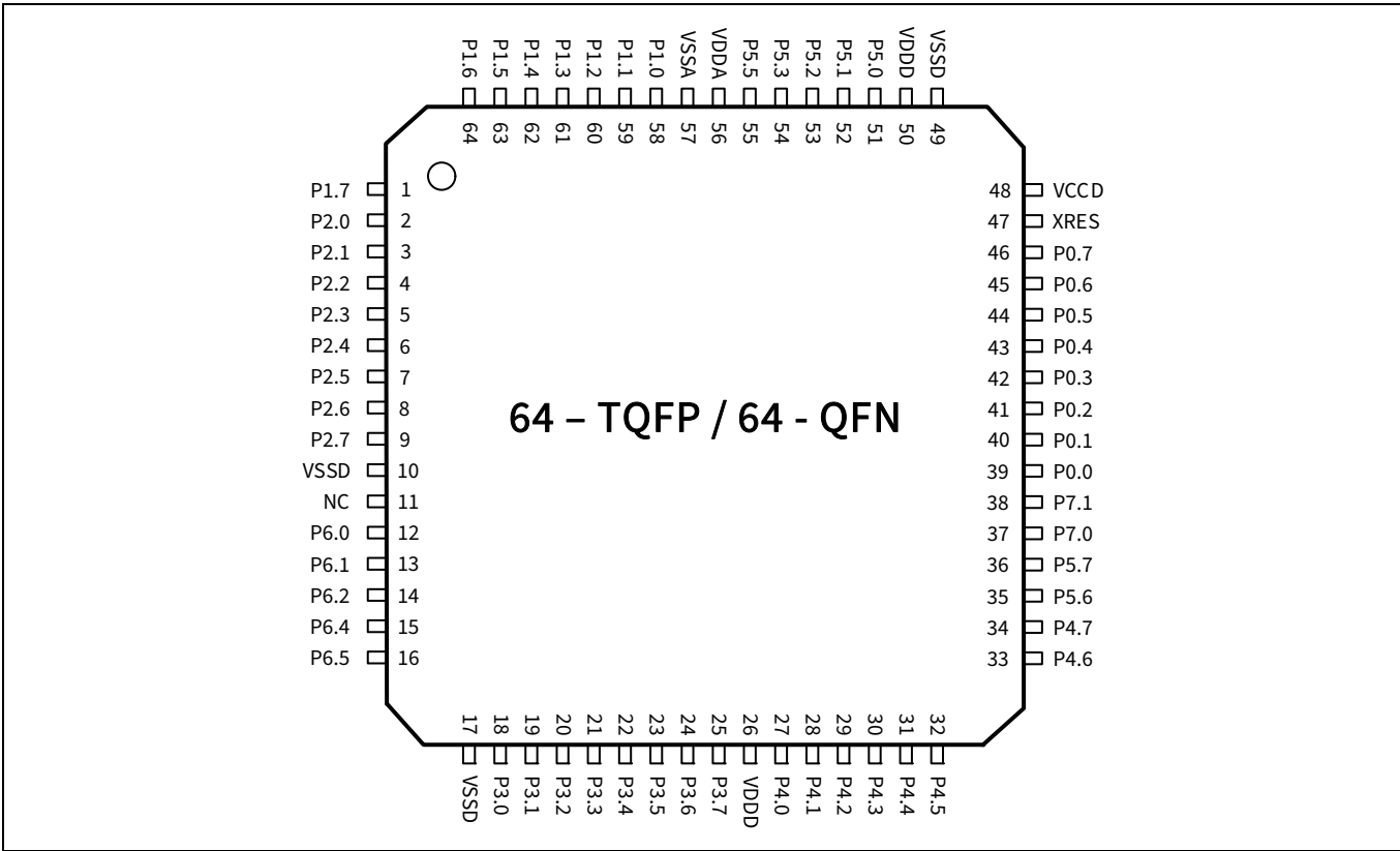
Figure 7 64-pin QFN and 64-pin TQFP pinout
