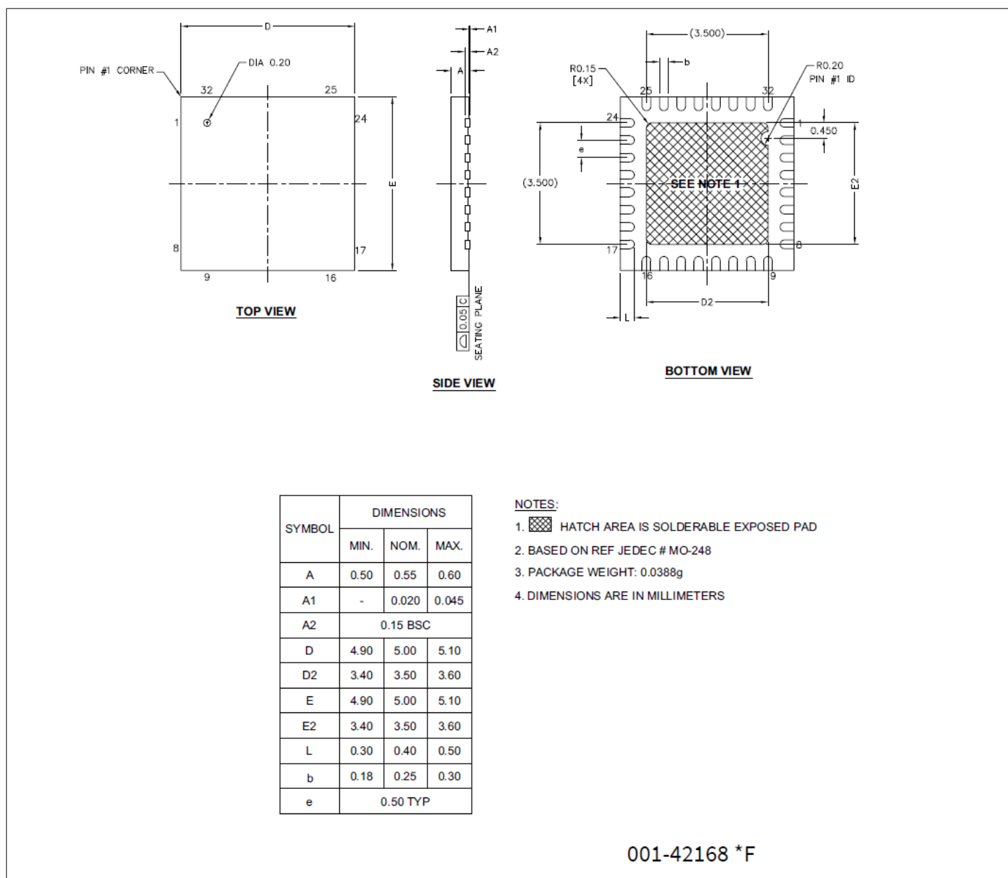
Figure 11 32 LEAD QFN 5.0x5.0x0.55 MM LQ32/LQ32B 3.5x3.5 MM EPAD (SAWN) package outline (PG-VQFN-32), 001-42168
