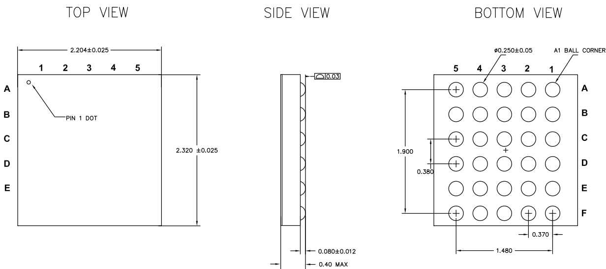
Figure 21. 30-pin WLCSP
