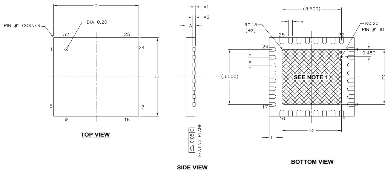
Figure 19. 32-Pin (5 × 5 × 0.6 mm) QFN
