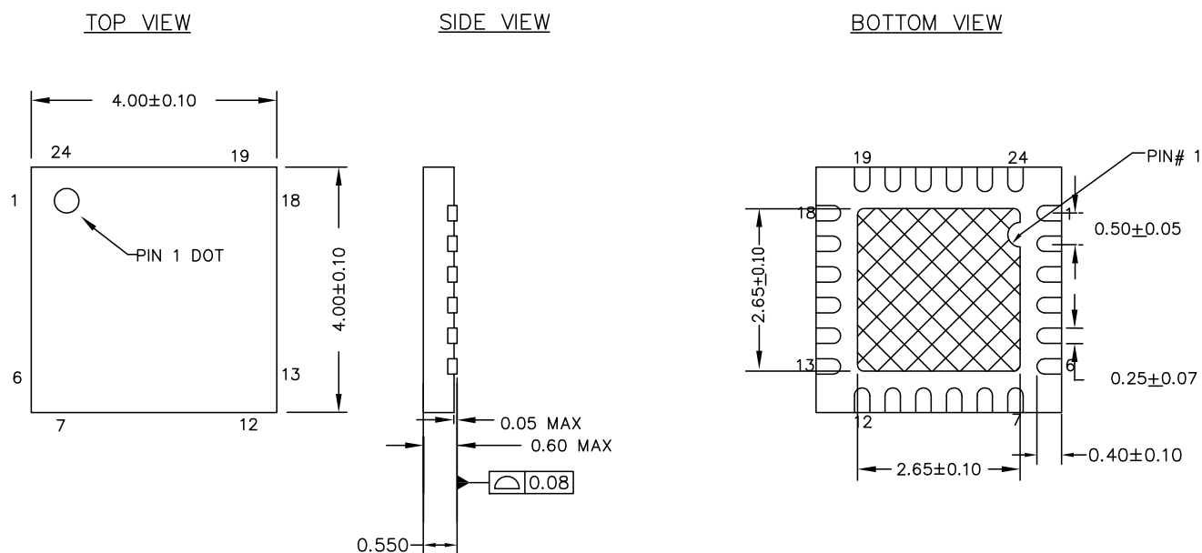
Figure 18. 24-Pin (4 × 4 × 0.6 mm) QFN
