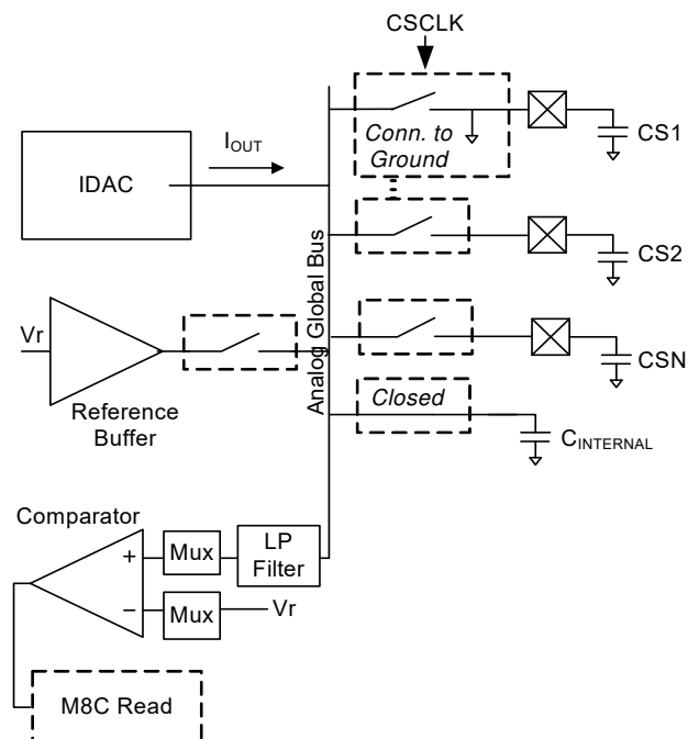
Figure 12-7. Second Phase of Successive Approximation
