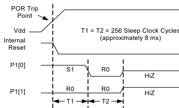
Figure 17-1. P1[1:0] Behavior on Power Up
