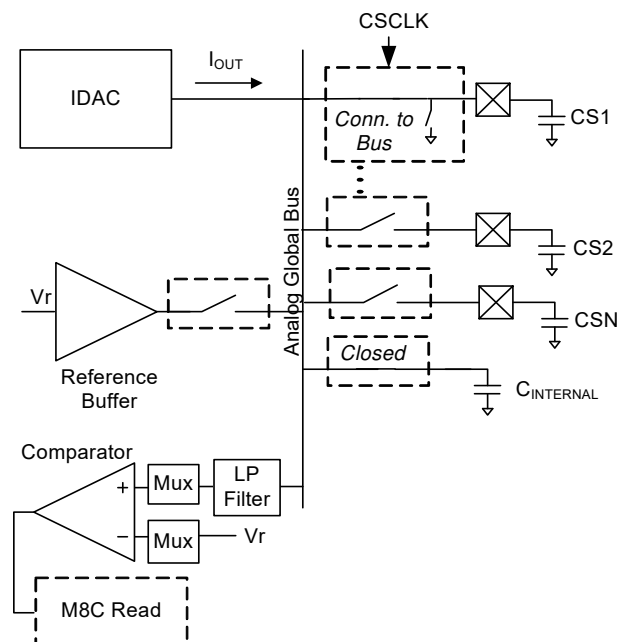
Figure 12-7. Second Phase of Successive Approximation
