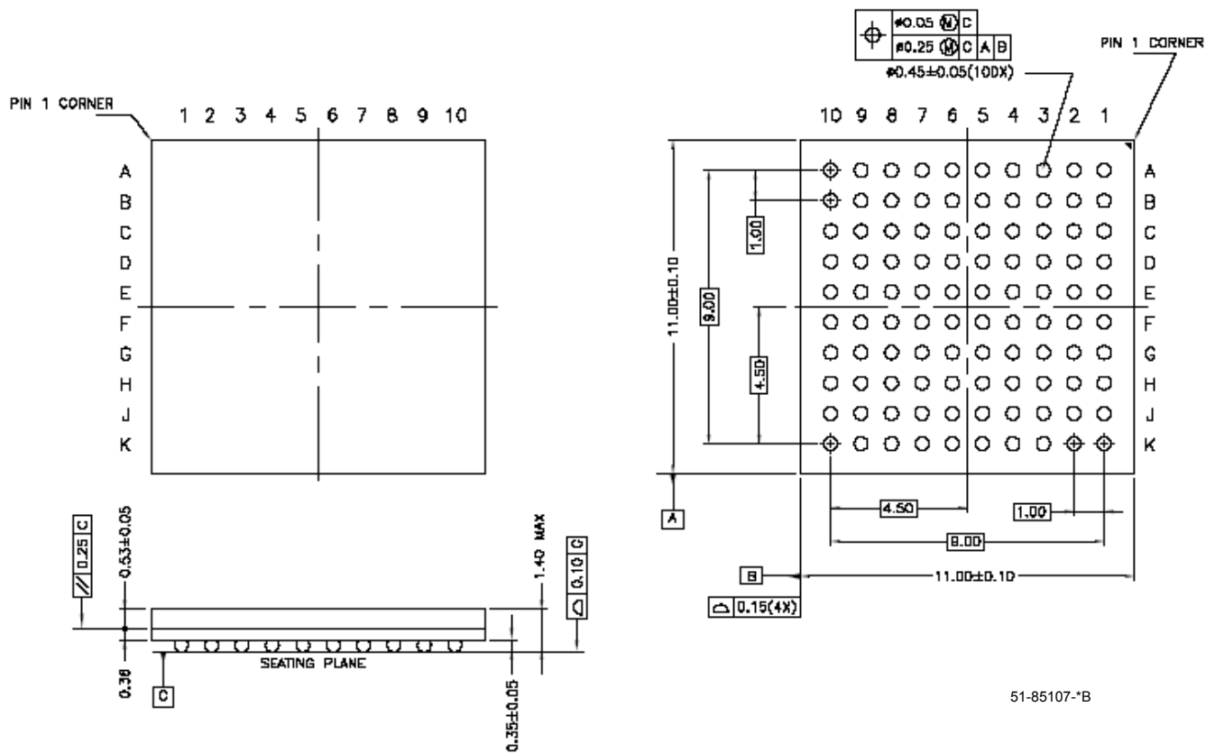
100-Ball Thin Ball Grid Array (11 x 11 x 1.4 mm) BB100
