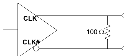
Figure 7. LVDS Termination
