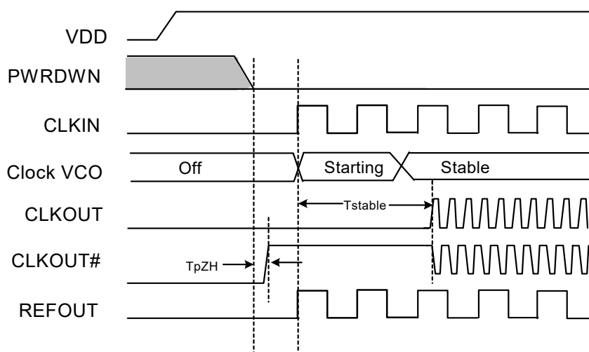
Figure 3. Power-down Deassertion
