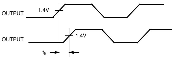
Figure 5. Input-Output Skew
