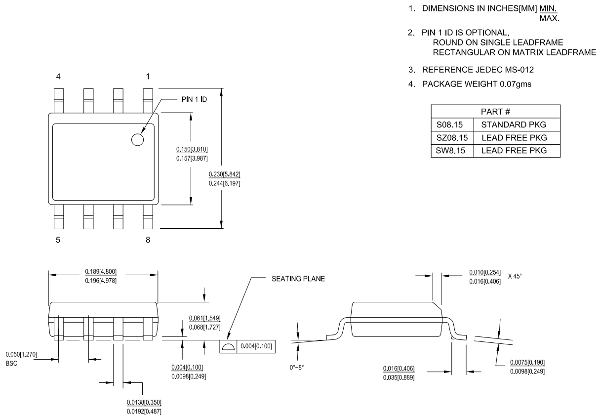
Figure 18. 8-pin SOIC (150 Mils) S08.15/SZ08.15 Package Outline, 51-85066
