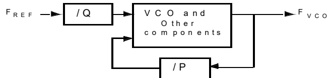
Figure 4. PLL system
