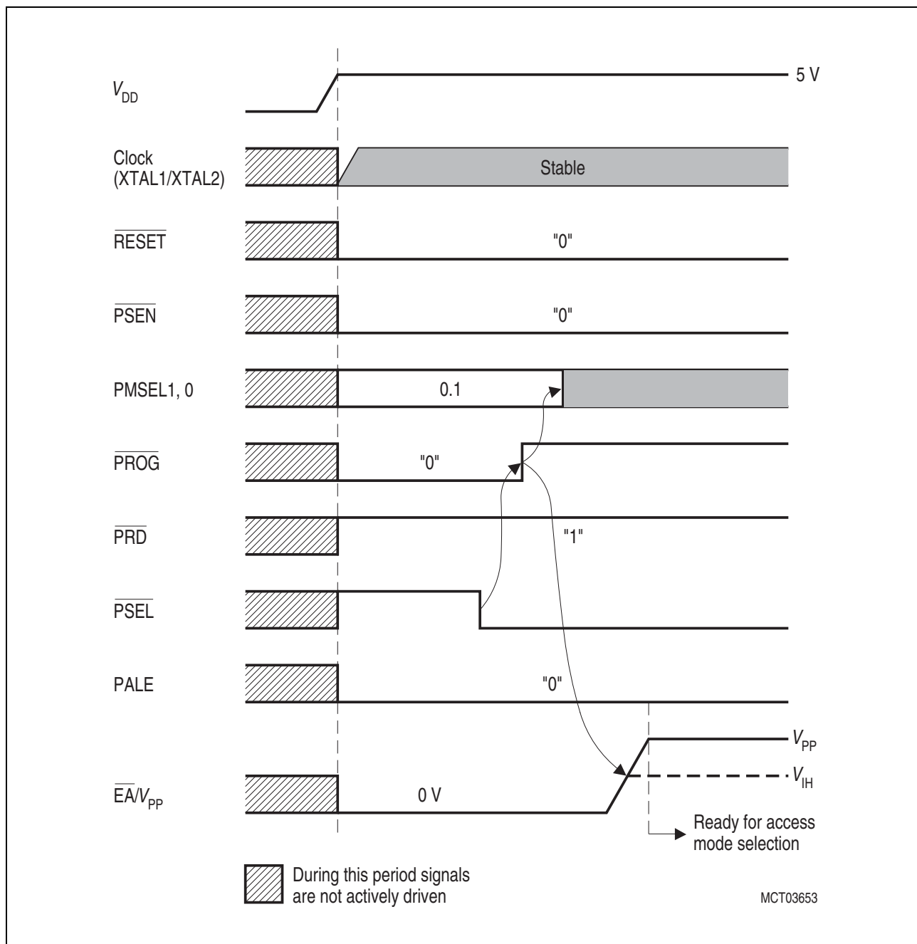
Figure 27 C515C-8E Basic Programming Mode Selection
