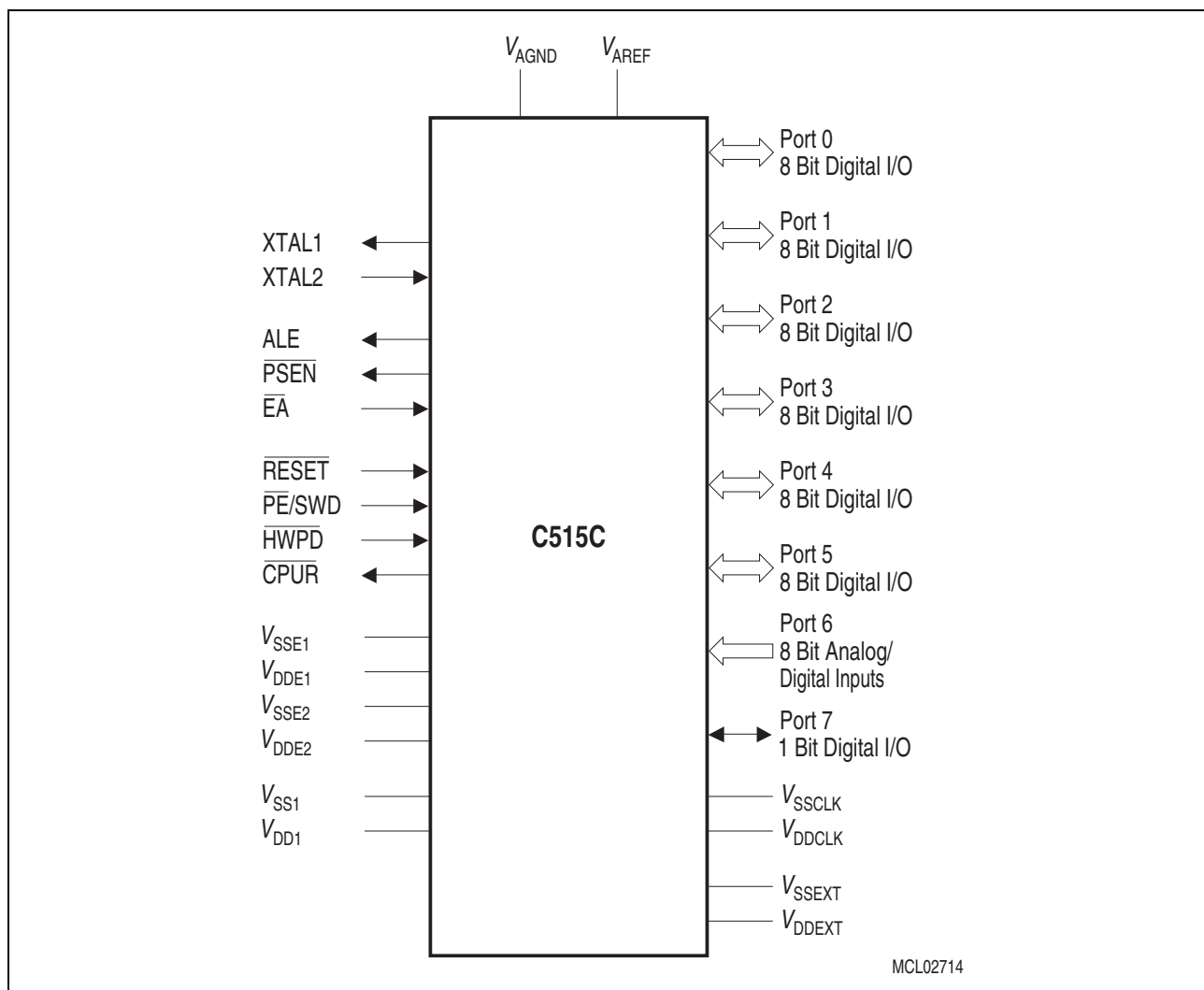
Figure 2 Logic Symbol
