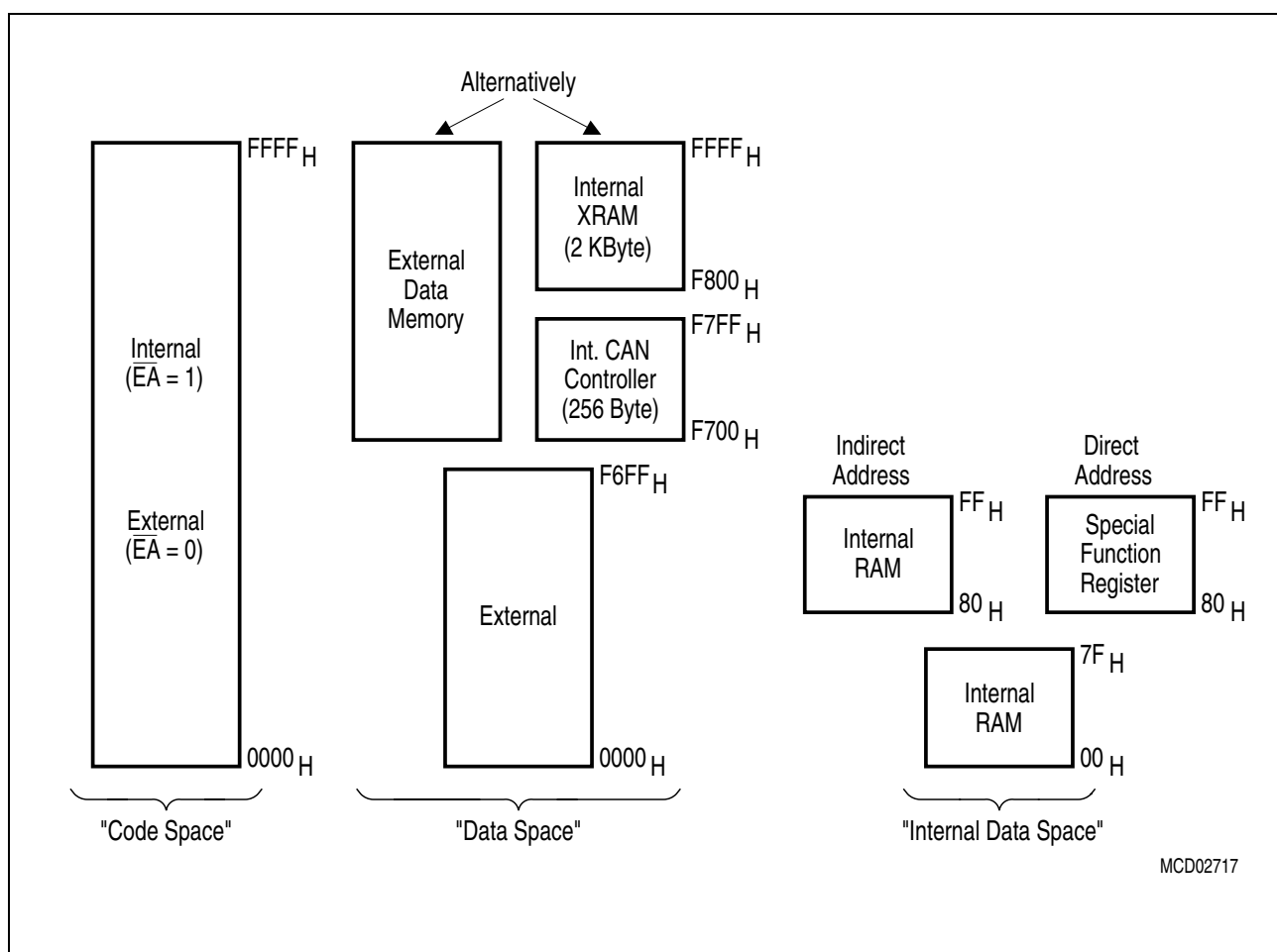
Figure 5 C515C Memory Map
