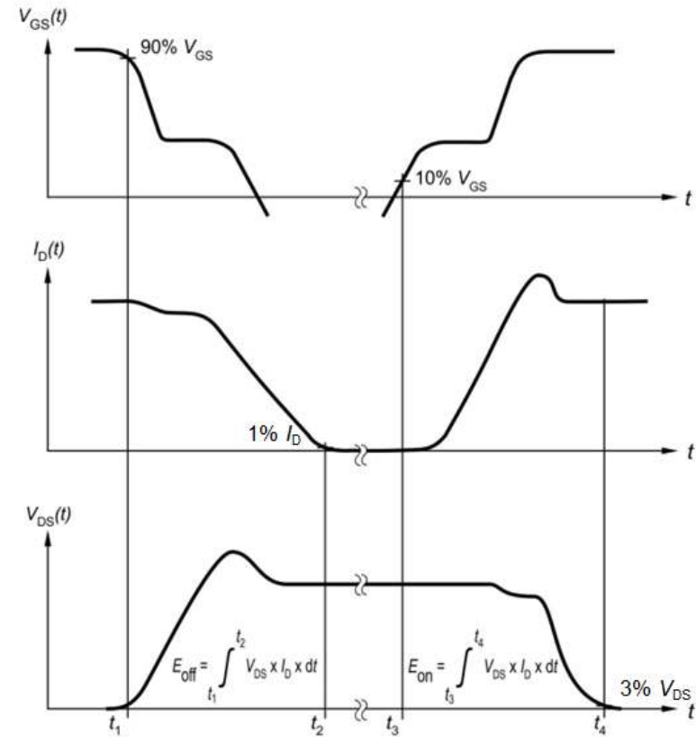
Figure B. Definition of switching losses
