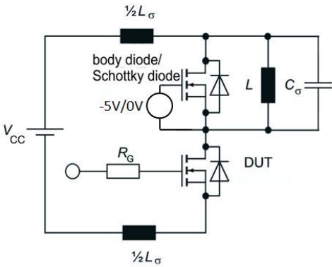
Figure E. Dynamic test circuit
