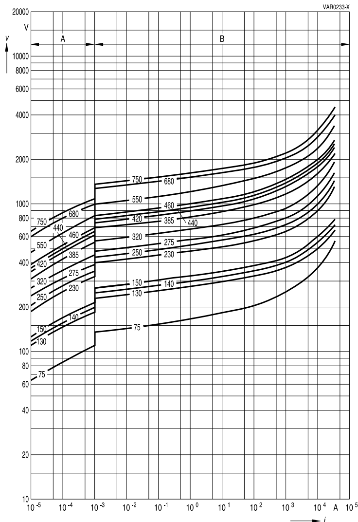
SIOV-B40K75 ... K750
