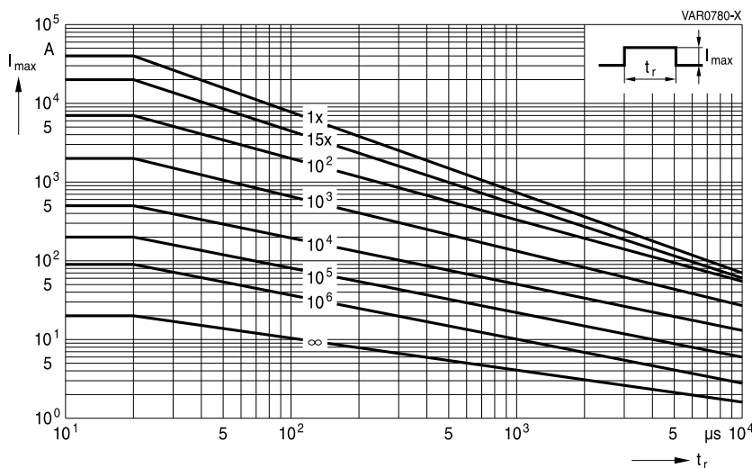
SIOV-LS40K230QP(K2) ... K460QP(K2)
