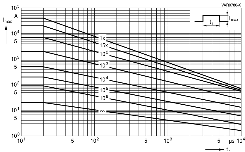
SIOV-LS40K230QP(K2) ... K460QP(K2)
