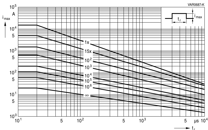
SIOV-Q20K350 ... K460
