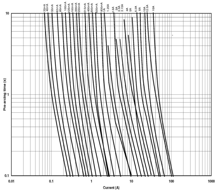
Nominal Time-Current Characteristics of S506-R
