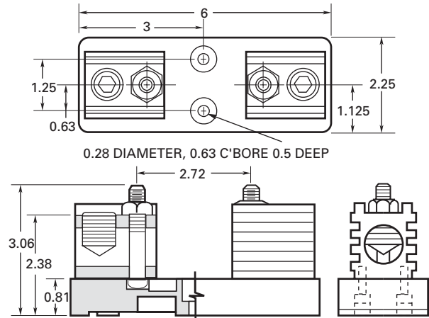
Figure 6. 201 to 400 A
