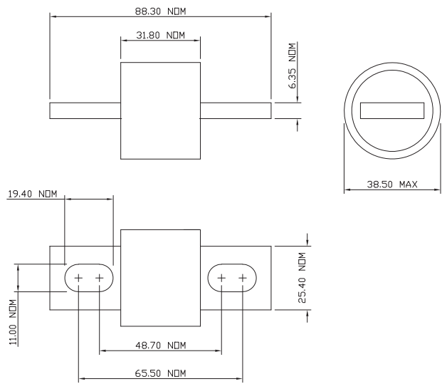
Dimensions - mm, 500 to 1000 A
