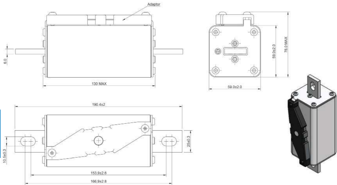
Dimensions - mm, size 2XL Bolted
