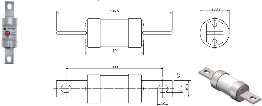
Dimensions - mm, TF125 to TF200
