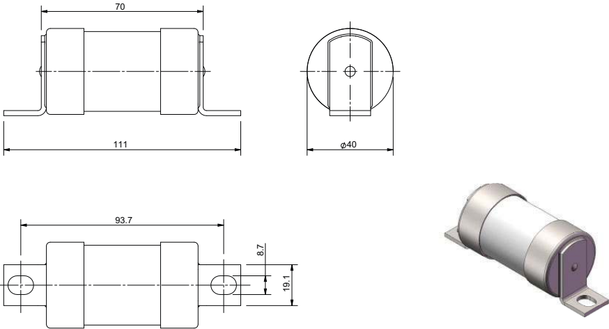
Dimensions - mm, TFP200M250
