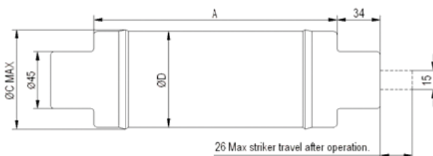
Dimensions - SJ Outline
