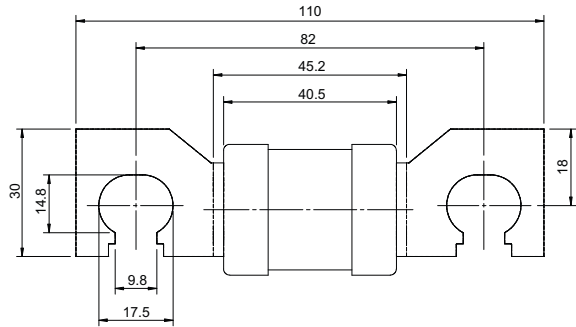
Dimensions - mm, up to 200 A
