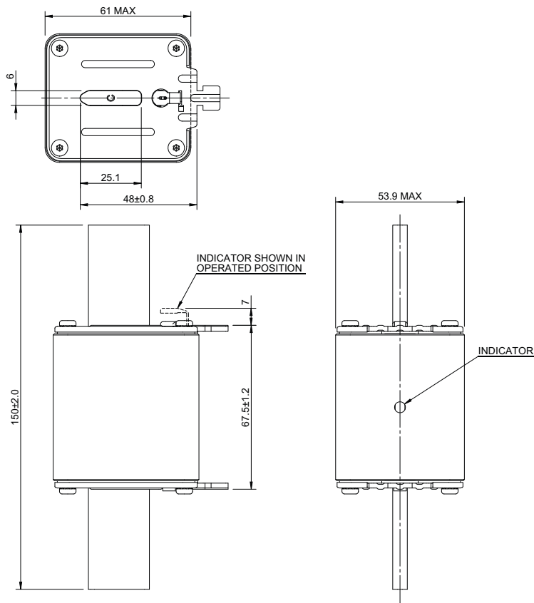
Dimensions - mm, NH2 Bladed fuse links
