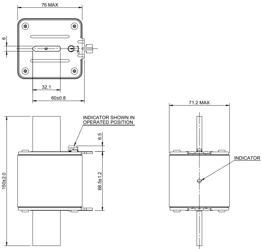
Dimensions - mm, NH3 Bladed fuse links
