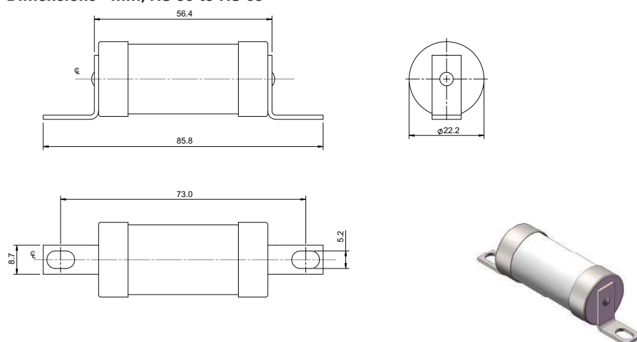
Dimensions - mm, TIS63M80 and TIS63M100
