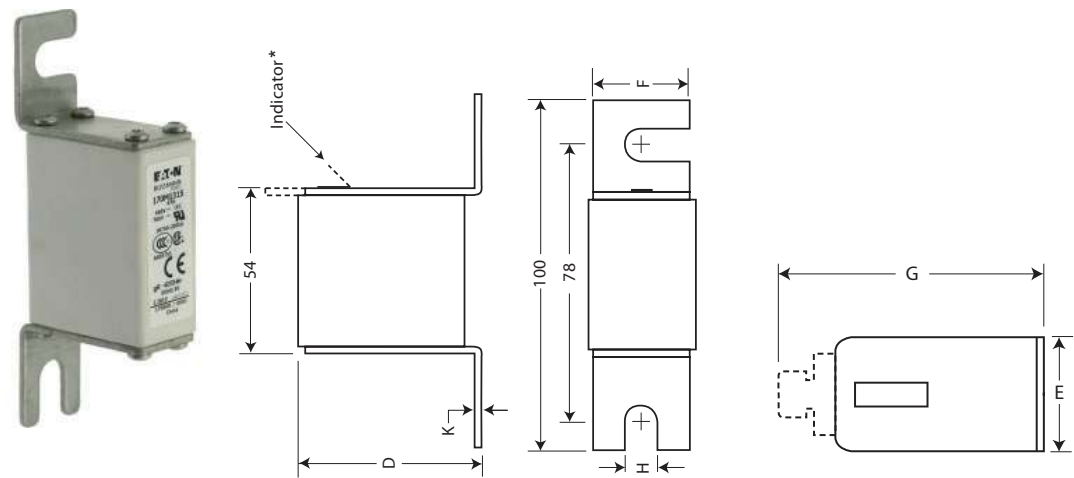
Dimensions - mm
