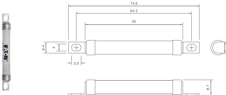
Dimensions - mm, CT
