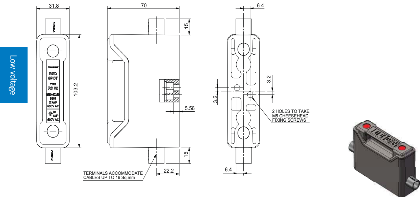
Dimensions - mm, RS32P 32 A Back stud connected
