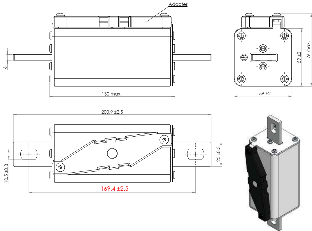
Dimensions - mm, size 2XL-3B Bolted
