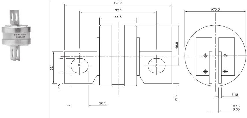
Dimensions - mm
