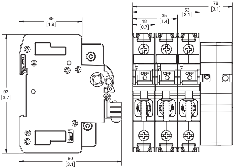
Dimensions - mm (inches), Side right rotary switch
