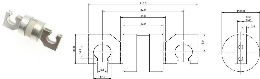
Dimensions - mm
