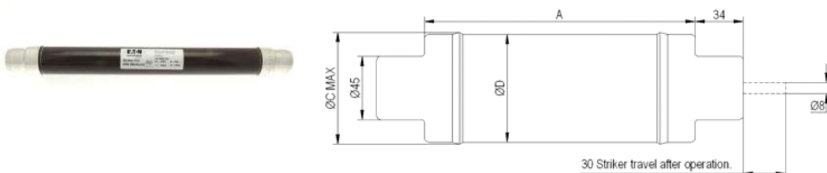
Dimensions - EJ Outline
