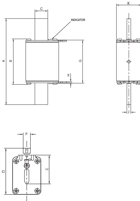
Dimensions - mm
