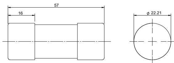
Dimensions - mm
