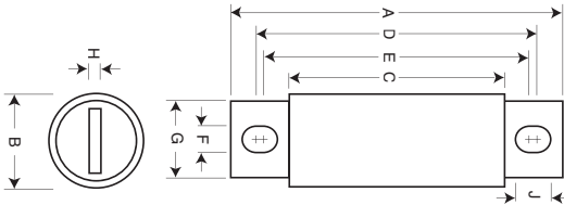
Dimensions - inches, 35 to 800 A
