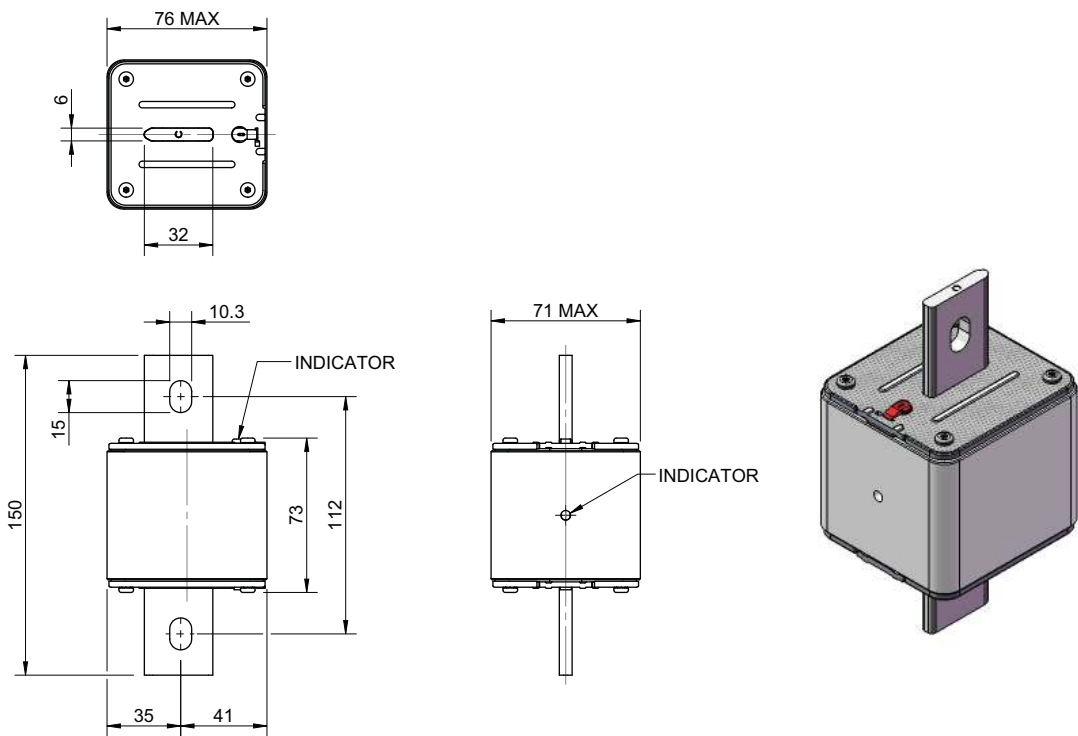
Dimensions - mm, NH3 Blade with bolt holes
