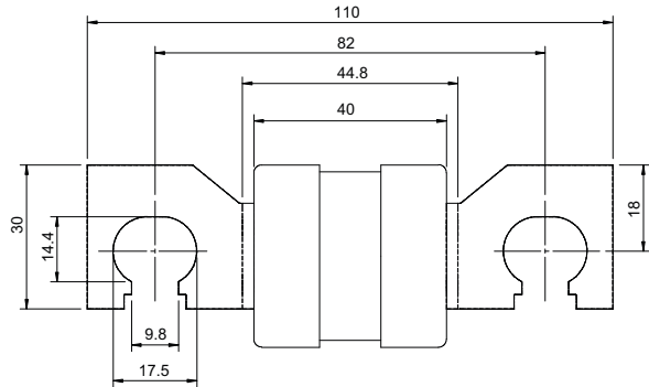
Dimensions - mm, 250 A and 315 A
