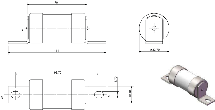
Dimensions - mm, TFP125 to TFP200
