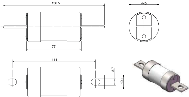
Dimensions - mm, TF200M250 and TF200M315
