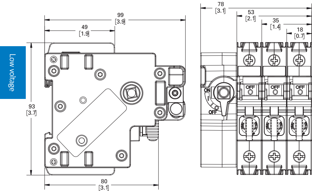
Dimensions - mm (inches), Front left rotary switch
