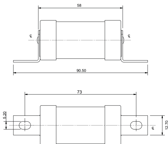
TIS63M80 and TIS63M100
