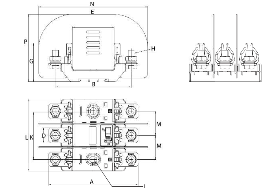
Dimensions - mm, 3-pole integral size 00
