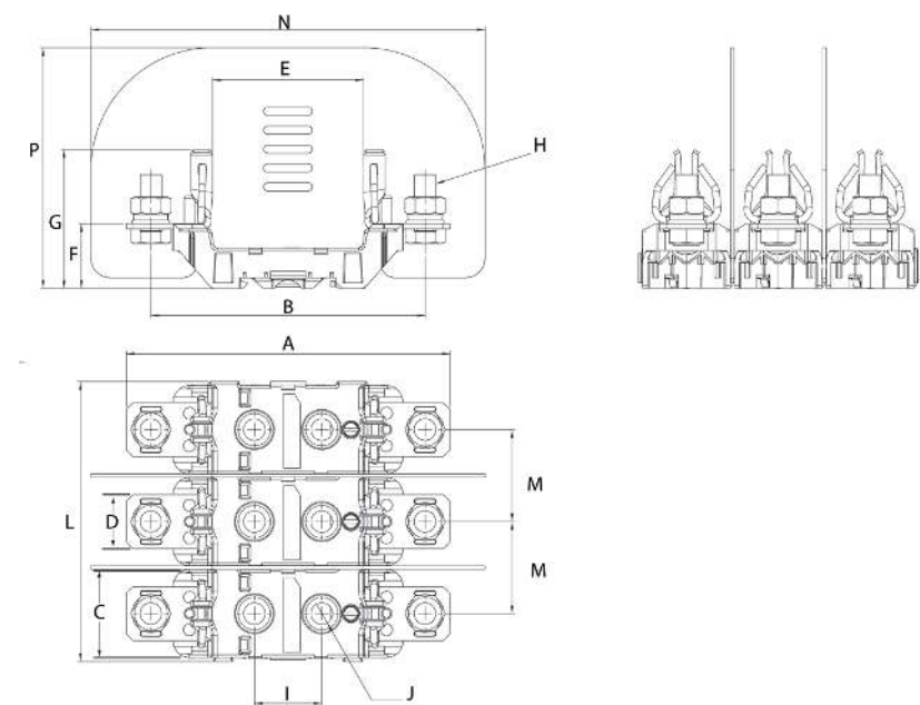
Dimensions - mm, 3-pole size 00
