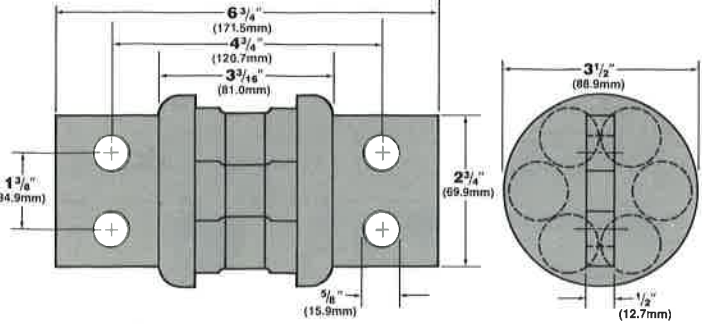
900-1000 Ampere Rating
