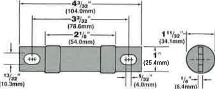
125-200 Ampere Rating
