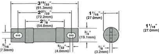
70-100 Ampere Rating
