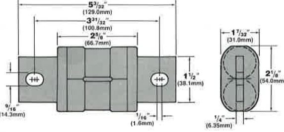
250-400 Ampere Rating
