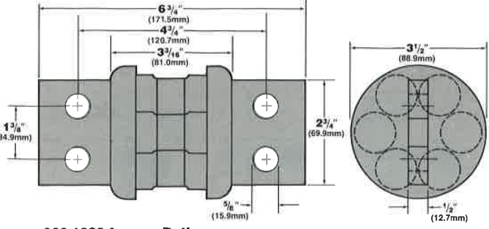
900-1000 Ampere Rating
