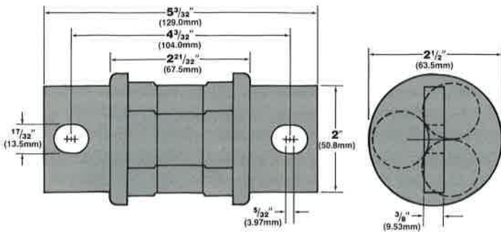
450-600 Ampere Rating
