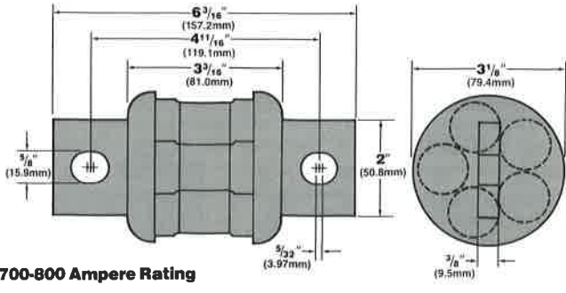
700-800 Ampere Rating
