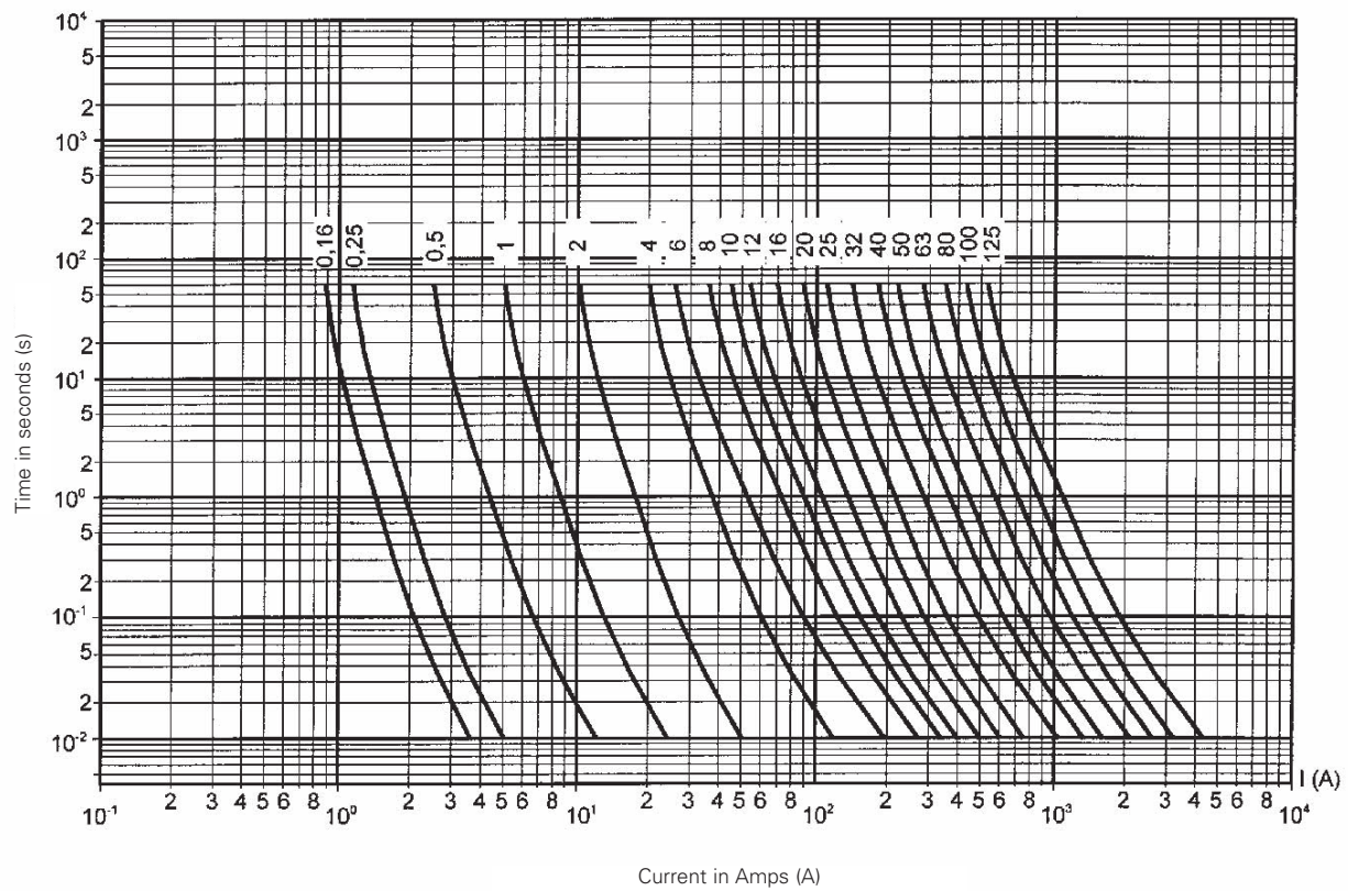
Time-current curves - Class aM
