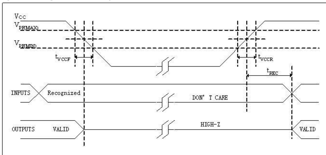
Figure 1. Power-Up/Power-Down Timing
