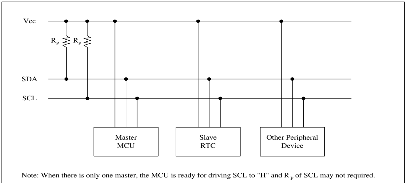
Figure 1. System Configuration
