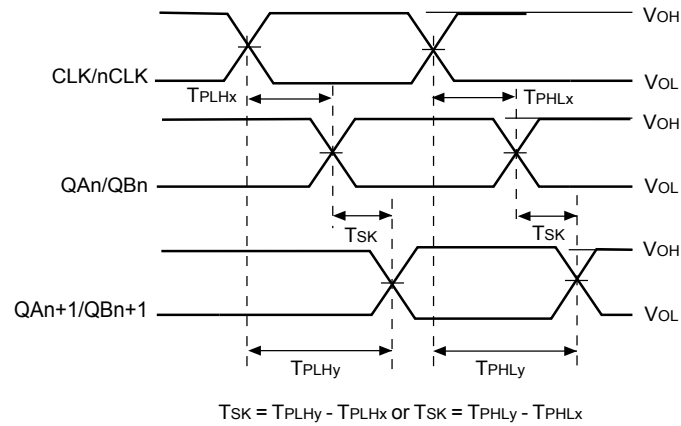
Figure 1. Output Skew
