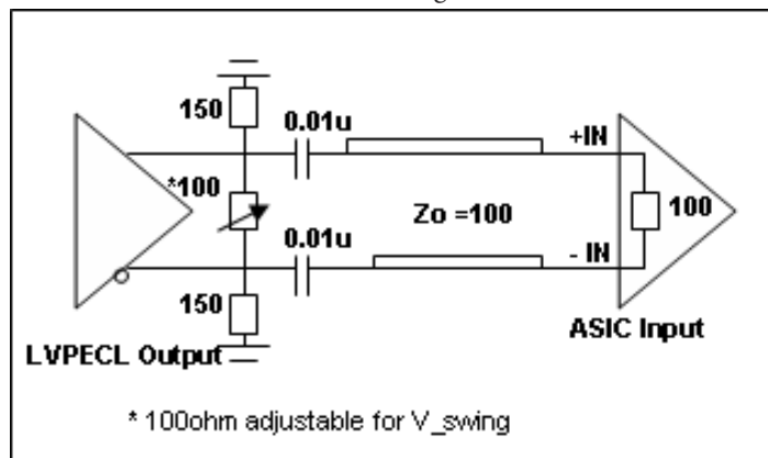
LVPECL Output V_{\text{swing}} Adjustment
