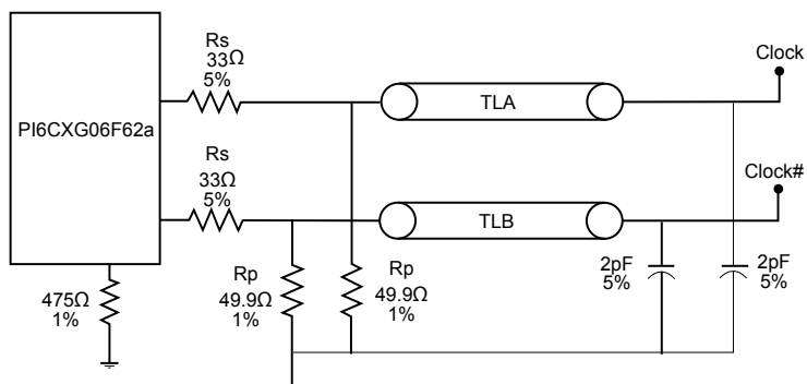
Figure 2. Configuration Test Load Board Termination for HCSL Outputs
