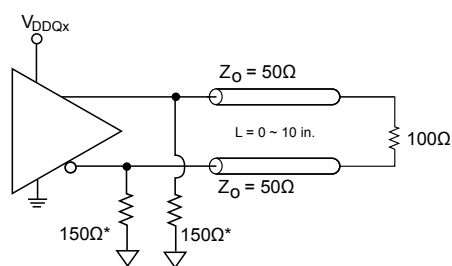
Figure 3. Configuration Test Load Board Termination for LVPECL/ LVDS Outputs
