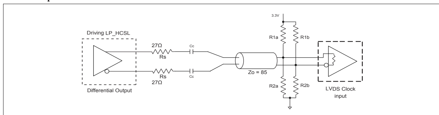
Figure 3. Differential Output Driving LVDS
