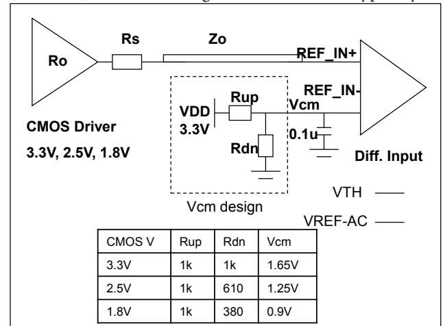
Fig 7: CMOS DC Input Vcm Design
