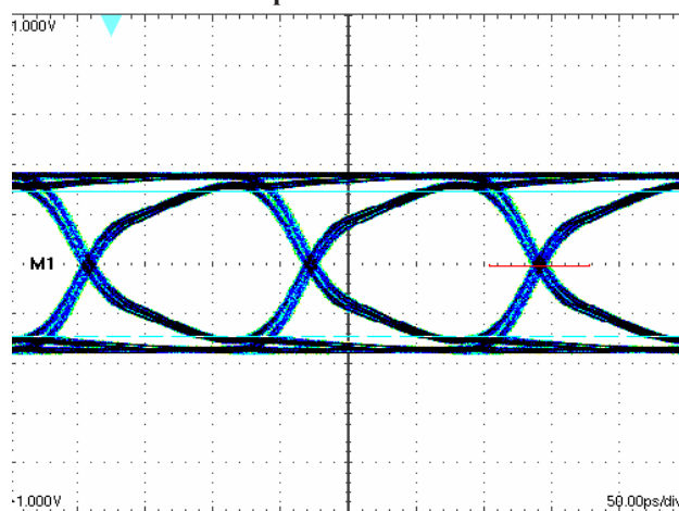
6Gb/s SATA CML output waveform
