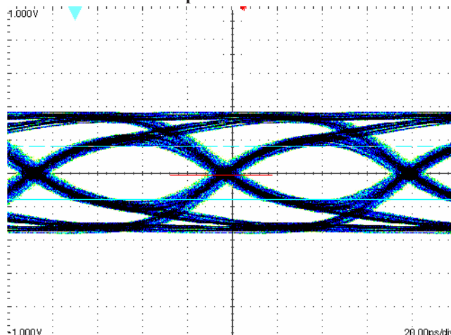
12Gb/s SATA CML output waveform
