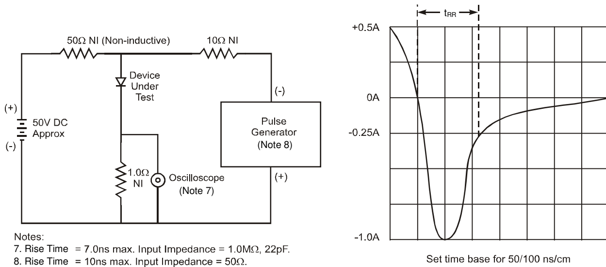
Figure 6. Reverse Recovery Time Characteristic and Test Circuit
